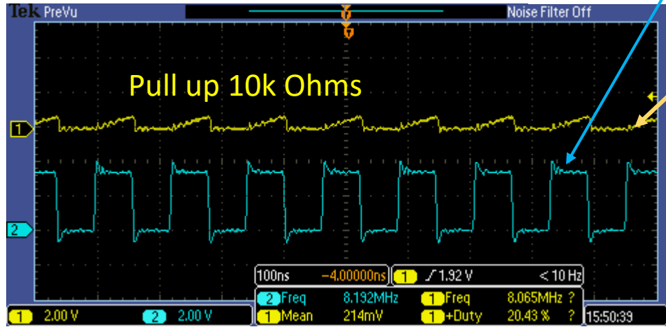
Fig. No.1: Input & output of SN74LVC04A with 10K pull-up
