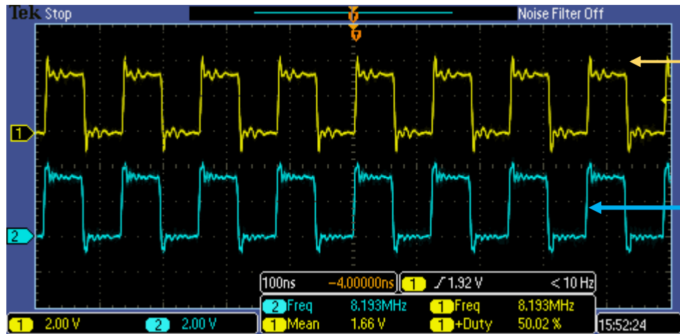
Fig. No.3: Input & Output of 74LVC125
