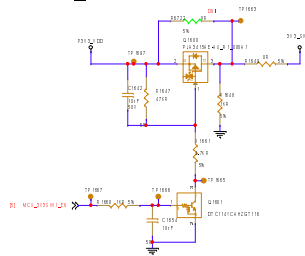
3V3_SW1
