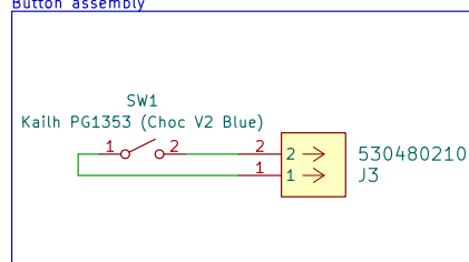
Button assembly
