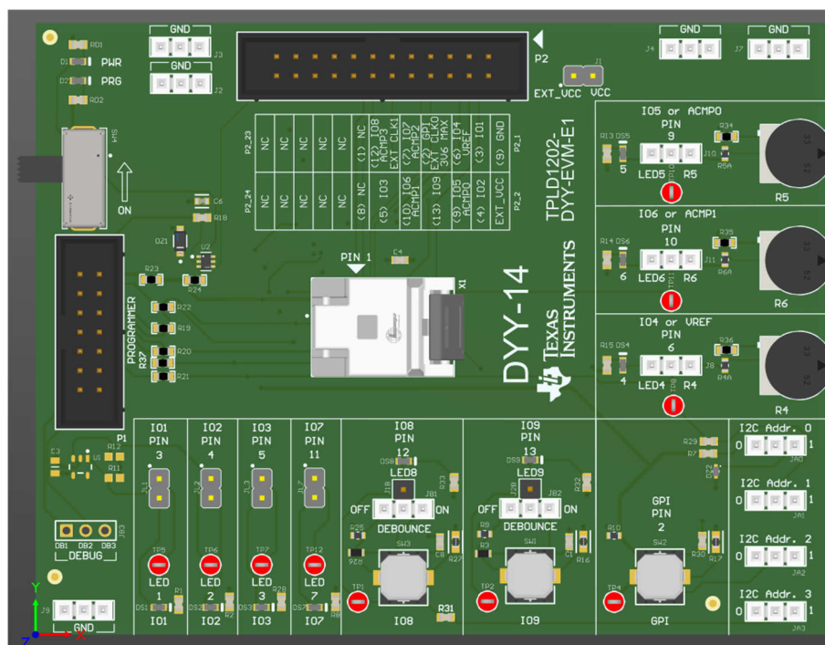
Figure 4-5. TPLD1202-DYY-EVM Board Front
