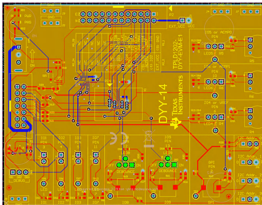
Figure 4-4. TPLD1202-DYY-EVM Layout
