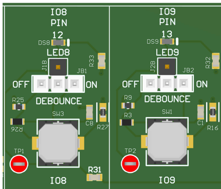
Figure 2-6. SW/LED Blocks
