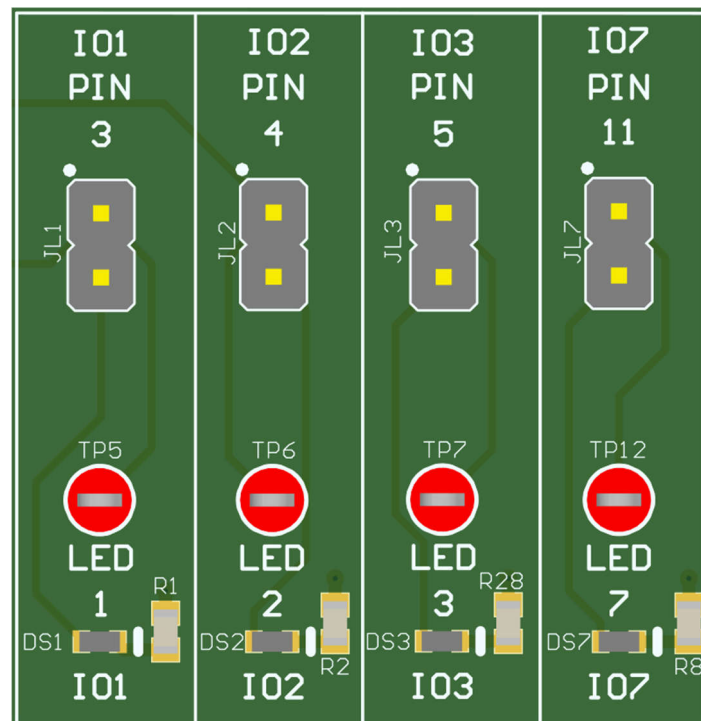
Figure 2-5. LED Blocks
