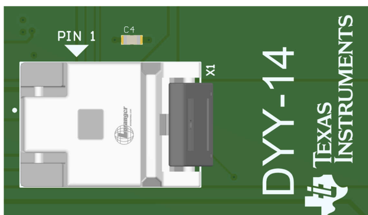
Figure 2-4. DYY Socket
