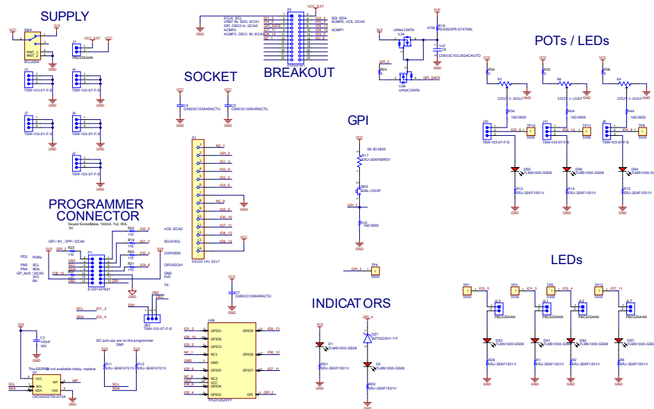
Figure 4-1. TPLD1202-DYY-EVM Schematic 1
