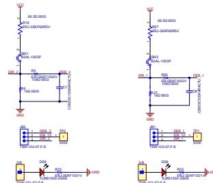
Figure 4-2. TPLD1202-DYY-EVM Schematic 2
