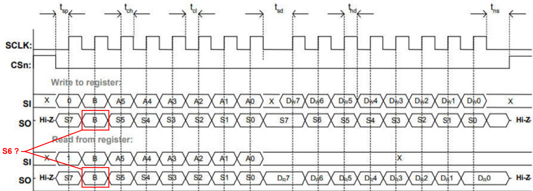
Figure 15: Configuration Registers Write and Read Operations
