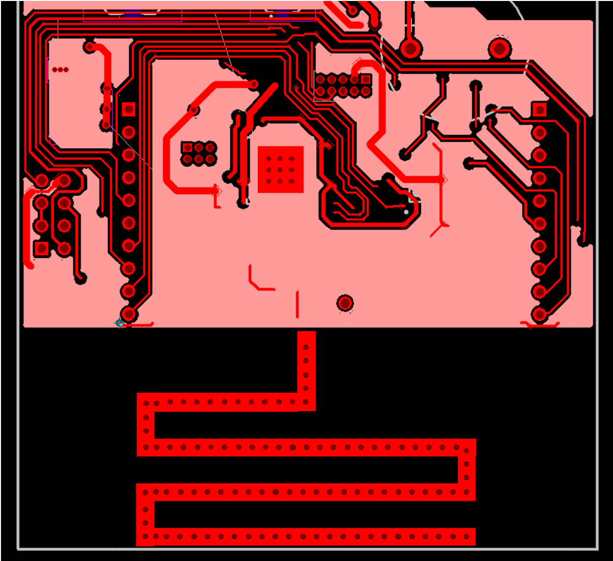
LAYER 2 with GND plane pink. Vias not visible
