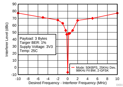
Figure 34. Rx Selectivity at 50 KBPS – 915 MHz
