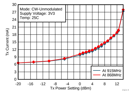
Figure 17. Tx Current vs Tx Power Setting – 868 MHz
