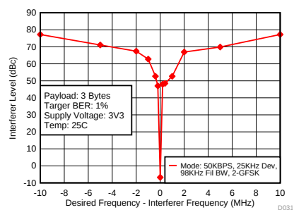
Figure 10. Rx Selectivity at 50 KBPS – 868 MHz
