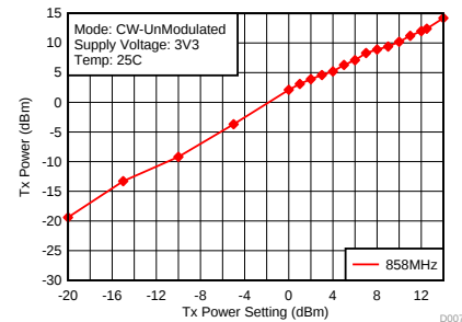
Figure 15. Tx Power vs Tx Setting – 868 MHz
