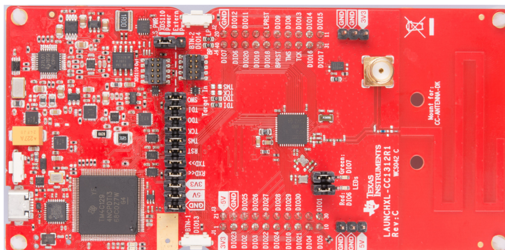
Figure 1. LAUNCHXL-CC1312R1 - Top side
