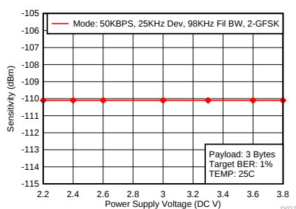
Figure 29. Rx Sensitivity vs Voltage at 50 KBPS – 915 MHz
