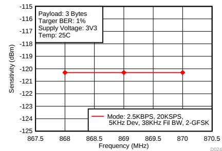
Figure 4. Rx Sensitivity vs Frequency in LRM – 868 MHz Band
