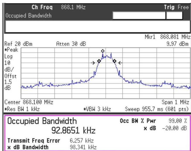
Figure 24. Tx Occupied Bandwidth at 50 KBPS at +14 dBm – 868 MHz
