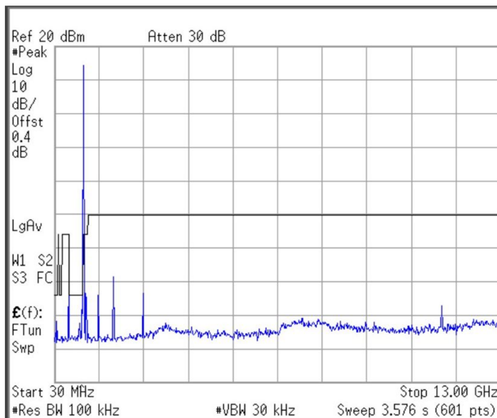
Figure 26. Tx Unwanted Emissions – Operating at 868 MHz - ETSI
