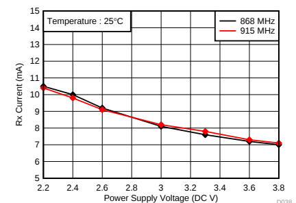
Figure 8. Rx Current vs Voltage in Rx Continuous Mode - 868 MHz
