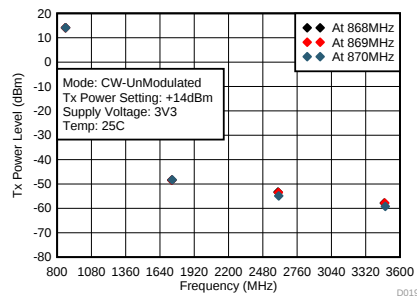
Figure 21. Harmonic Level at +14 dBm Setting – 868 MHz Band
