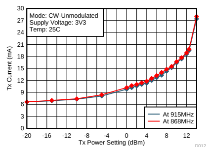
Figure 41. Tx Current vs Tx Power Setting - 915 MHz
