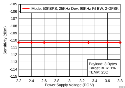
Figure 5. Rx Sensitivity vs Voltage at 50 KBPS – 868 MHz
