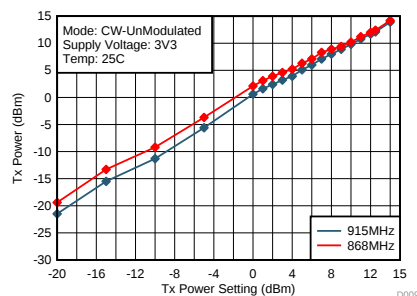
Figure 39. Tx Power vs Tx Power Setting - 915 MHz
