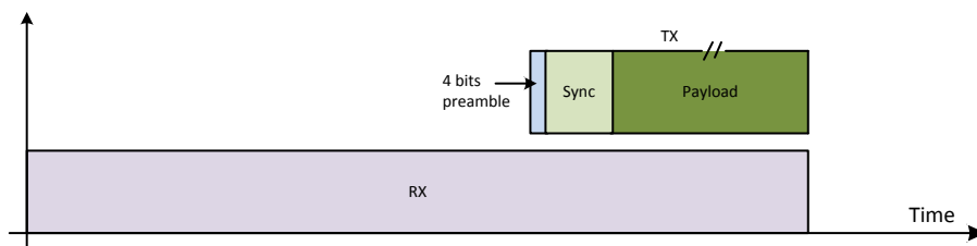
Figure 39: Ordinary RX Mode
