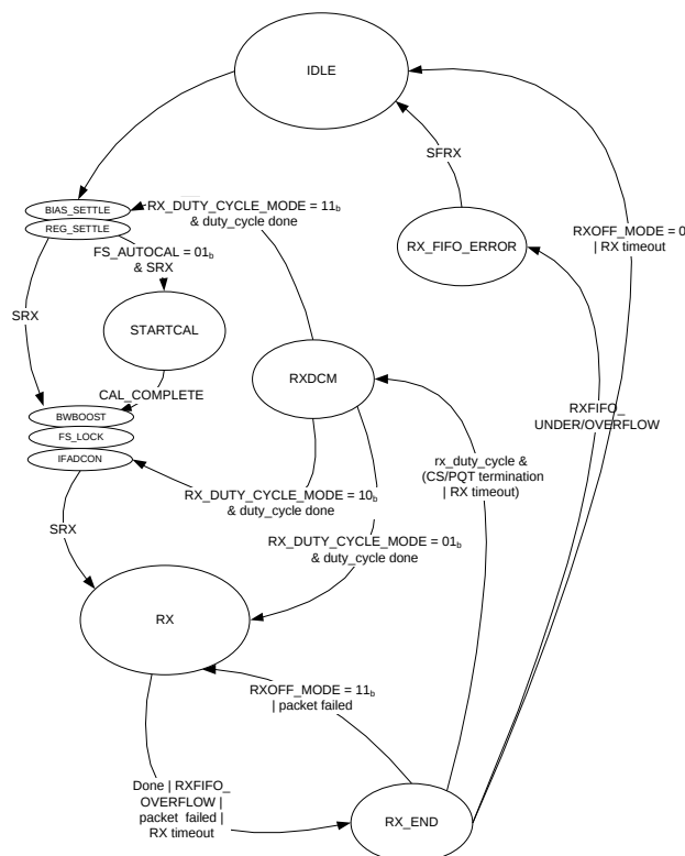
Figure 42: RXDCM State Diagram
