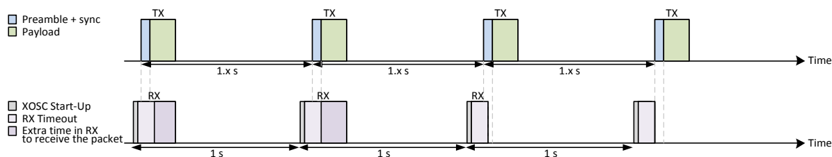
Figure 37: eWOR Mode (RX and TX out of sync.)
