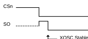
Figure 31: Power-On Reset
