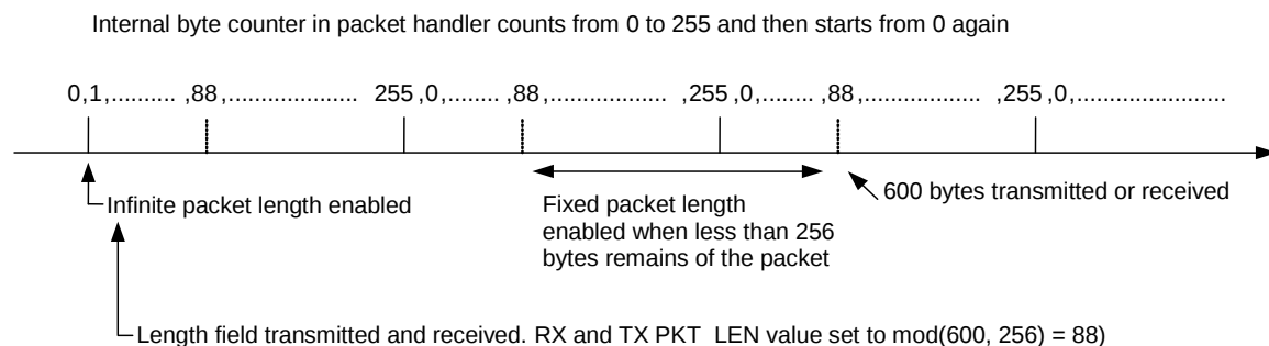
Figure 20: Packet Length > 255
