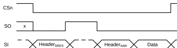
Figure 5: SRES Command Strobe
