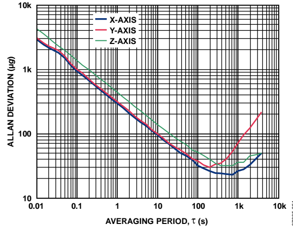
Figure 52. Root Allan Deviation
