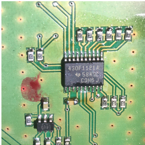
Picture of MSP430F1121A – on same board
