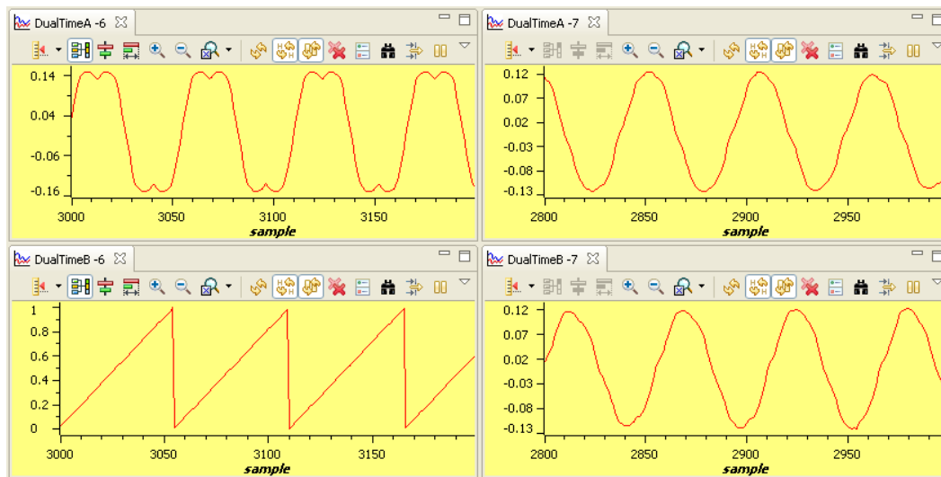
Fig 17 The waveforms of Sygen\_dq1.Ta , rg1.Out , and phase A&B currents*
