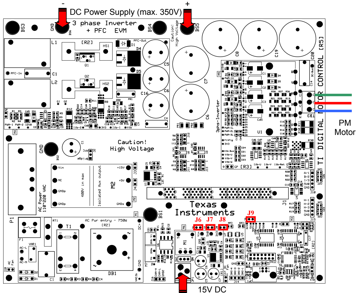
Fig. 12 Using External DC power supply to generate DC-Bus for the inverter
