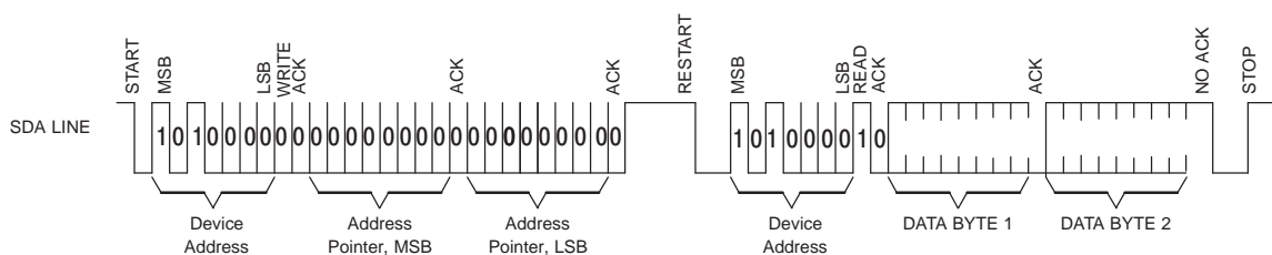
Figure 2-33. Random Read
