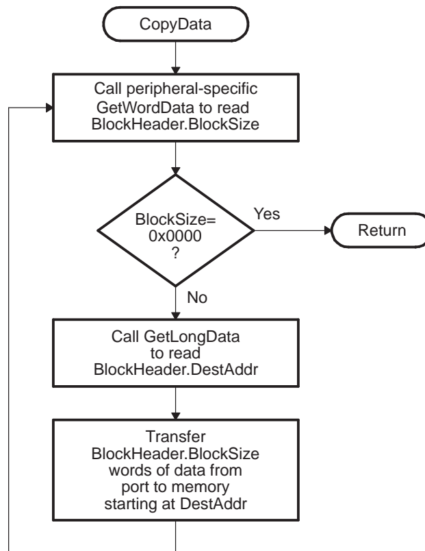
Figure 2-12. Overview of CopyData Function
