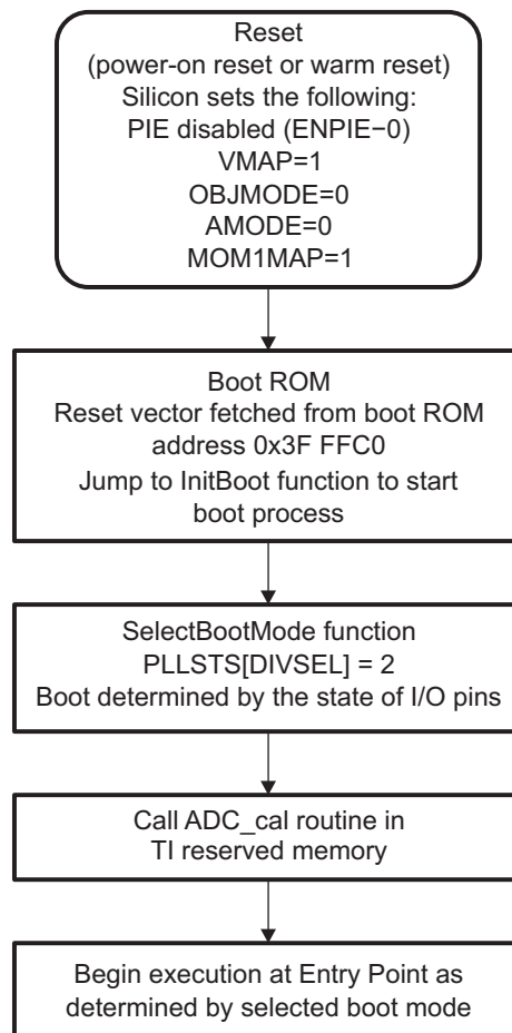
Figure 2-1. Bootloader Flow Diagram
