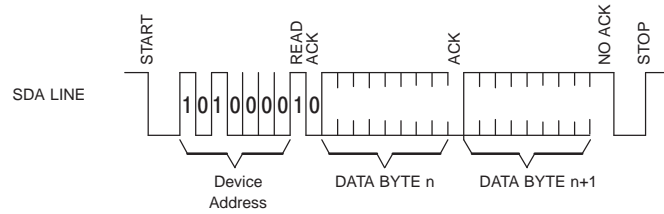
Figure 2-34. Sequential Read
