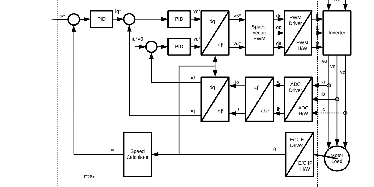
Figure 1 Field Oriented Control of PMSM
