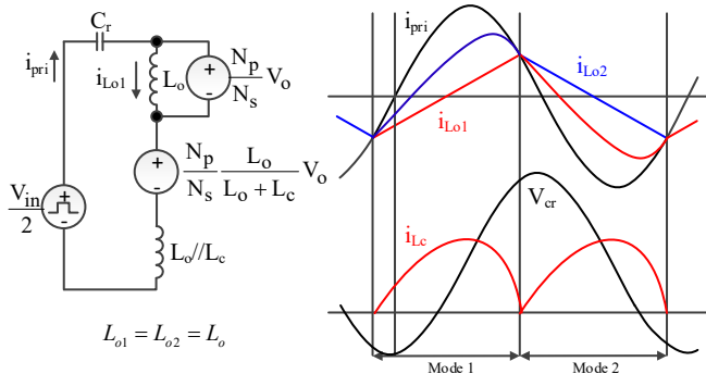
Fig. 8. Key waveforms of a resonant network
