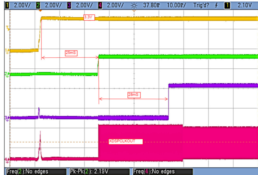
This shows XCLKOUT after 1.8V power up
