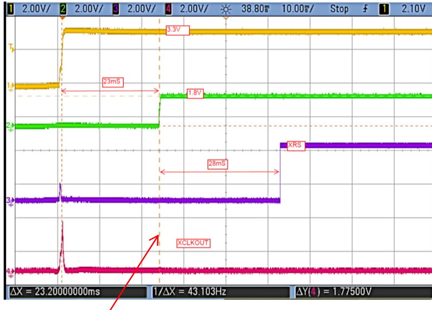
This shows NO XCLKOUT after 1.8V power up
