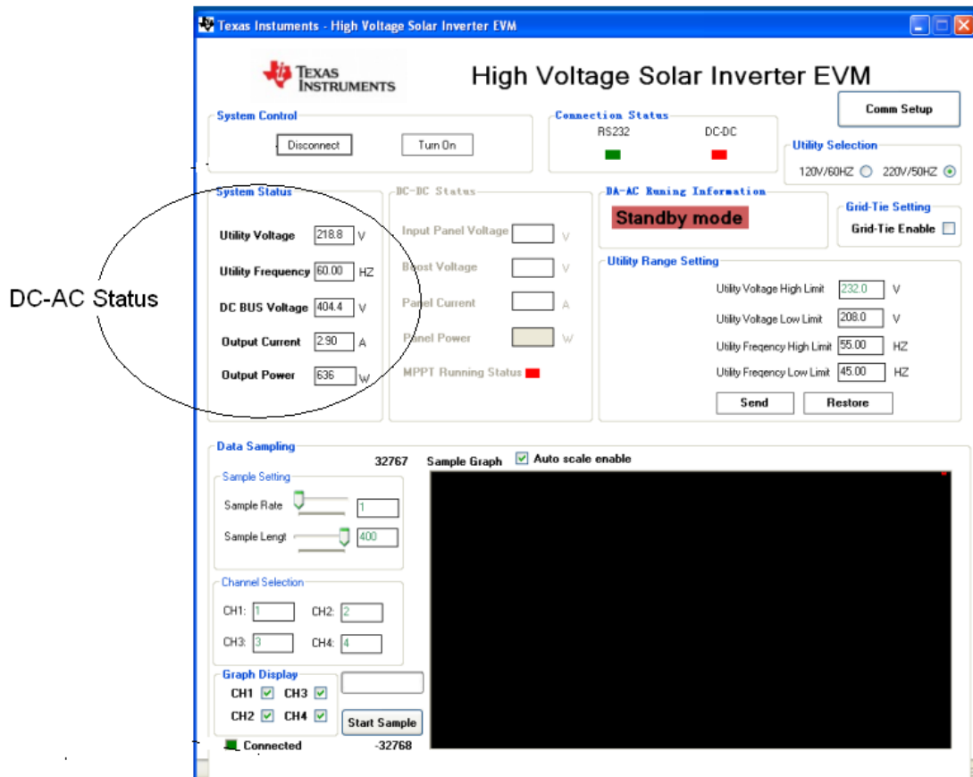
Fig 3.3 Check the DC-AC Status
