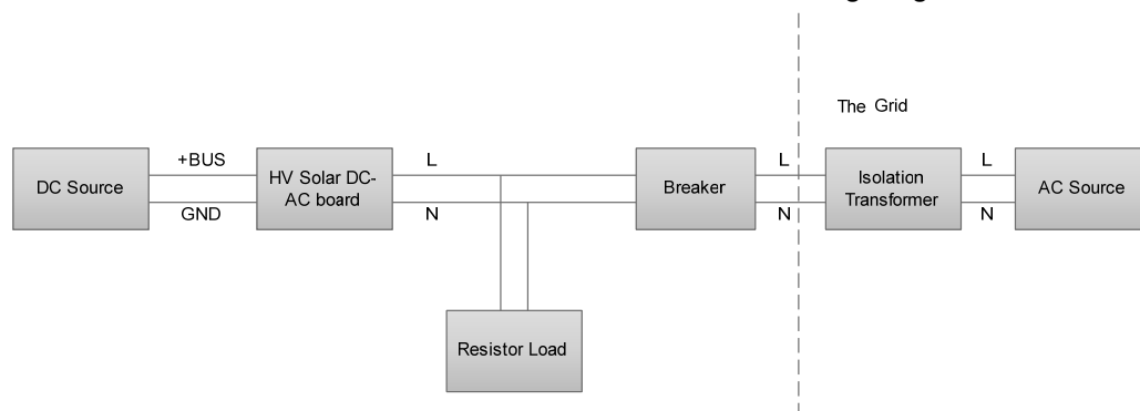
Fig 2.1 The connection of the test
