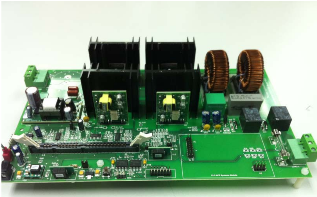
Figure1.1 Board Picture
