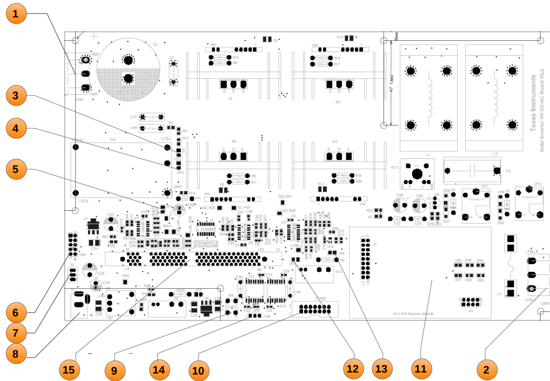
Fig 1.2 The Key Points of the Board
