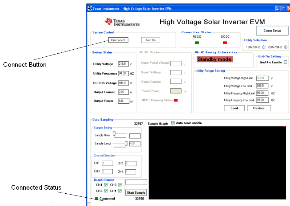
Fig 3.3 Connect the board
