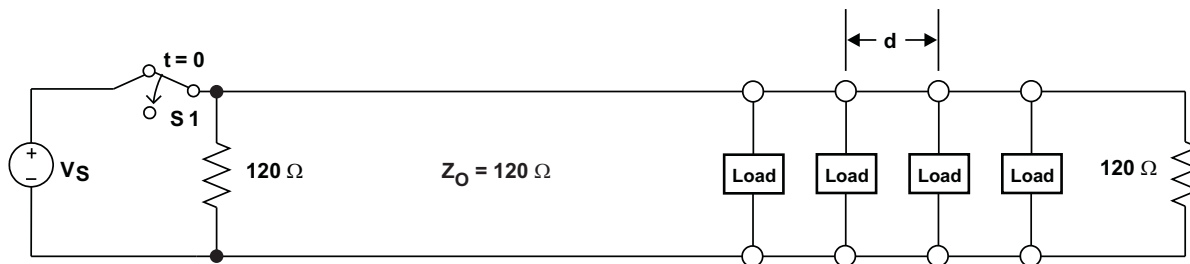
Figure 16. CAN Bus Schematic Diagram
