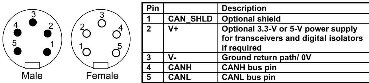
Figure 12. 5-Pin Mini-Connector (ANSI/B.93.55M-1981)
