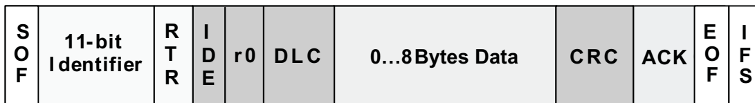
Figure 3. Standard CAN: 11-Bit Identifier
