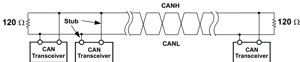
Figure 8. Standard Termination
