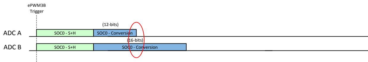
Figure 9-19. Example: Asynchronous Operation with Different Resolutions
