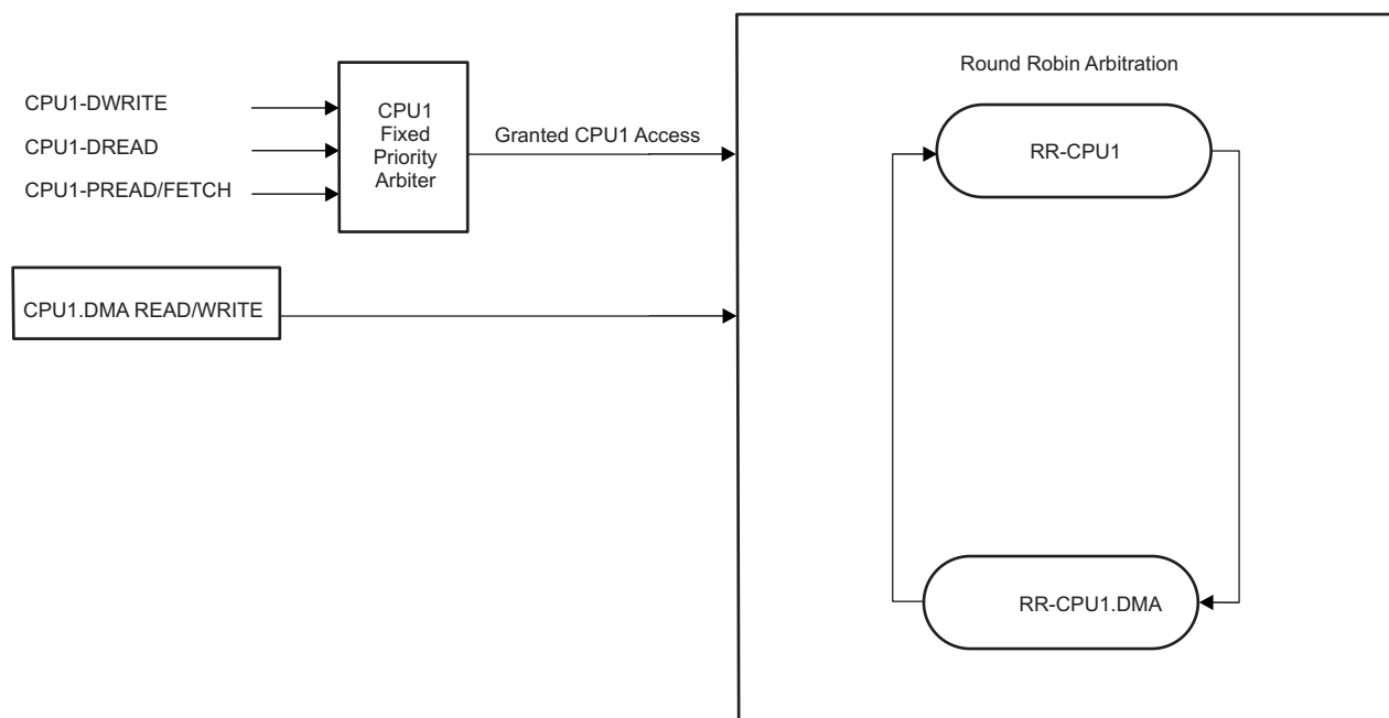
Figure 2-14. Arbitration Scheme on Global Shared Memories
