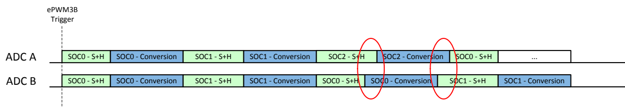
Figure 9-18. Example: Asynchronous Operation with Uneven SOC Numbers – Trigger Overflow
