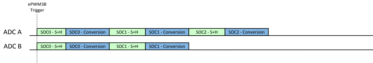
Figure 9-17. Example: Synchronous Operation with Uneven SOC Numbers
