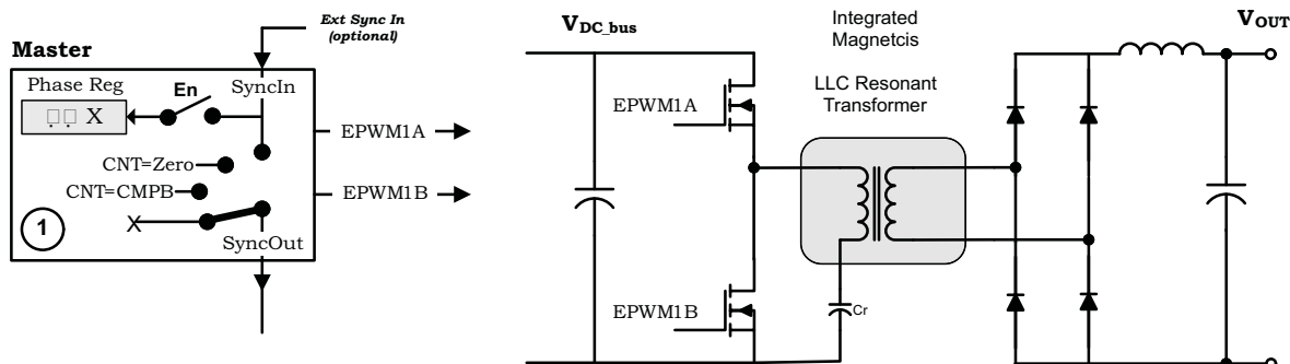
Figure 13-75. Control of Two Resonant Converter Stages
