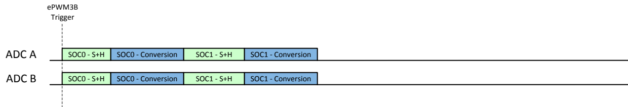
Figure 9-15. Example: Basic Synchronous Operation
