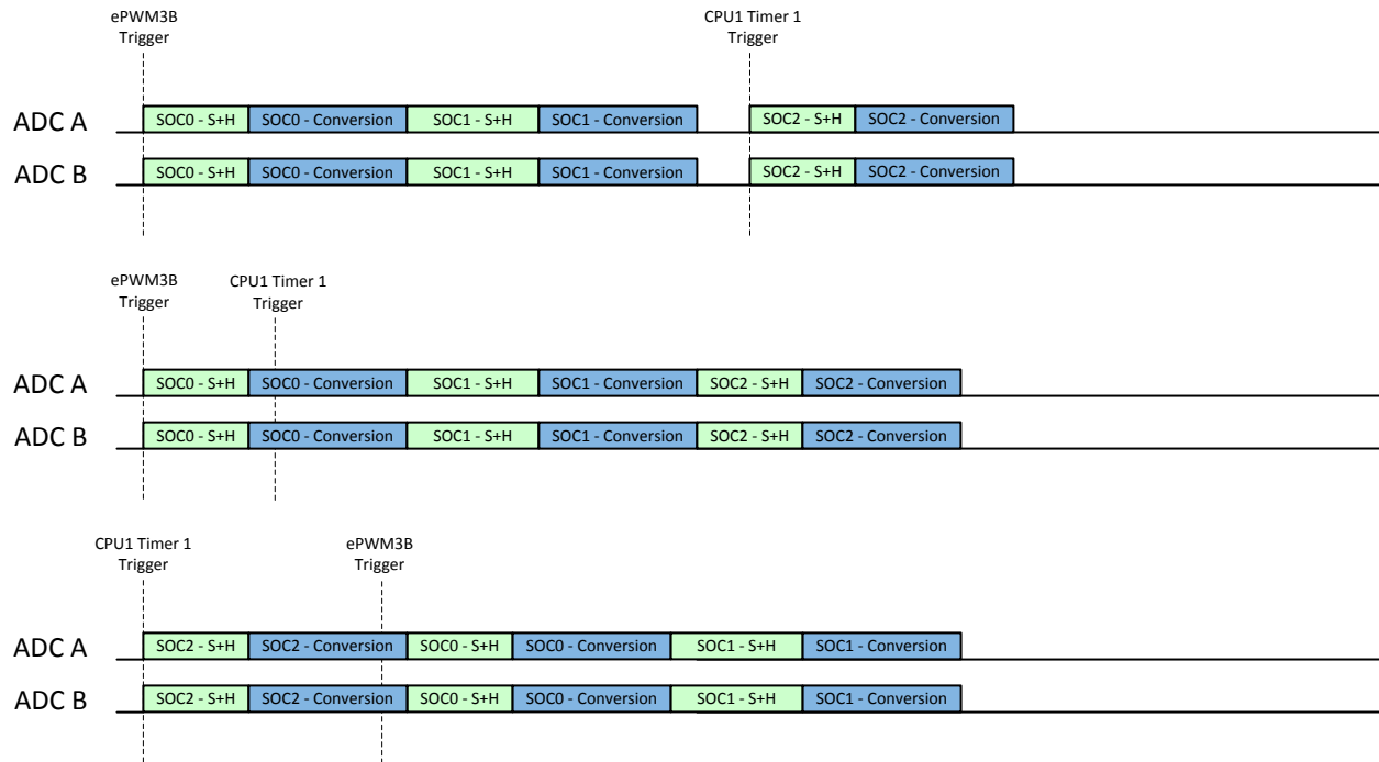
Figure 9-16. Example: Synchronous Operation with Multiple Trigger Sources
