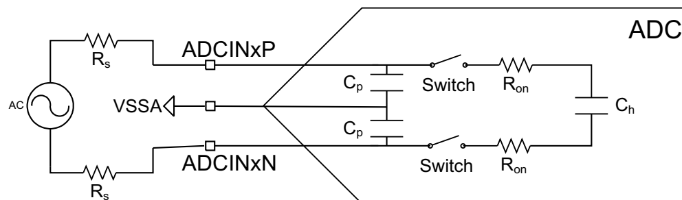
Figure 9-4. Differential Input Model
