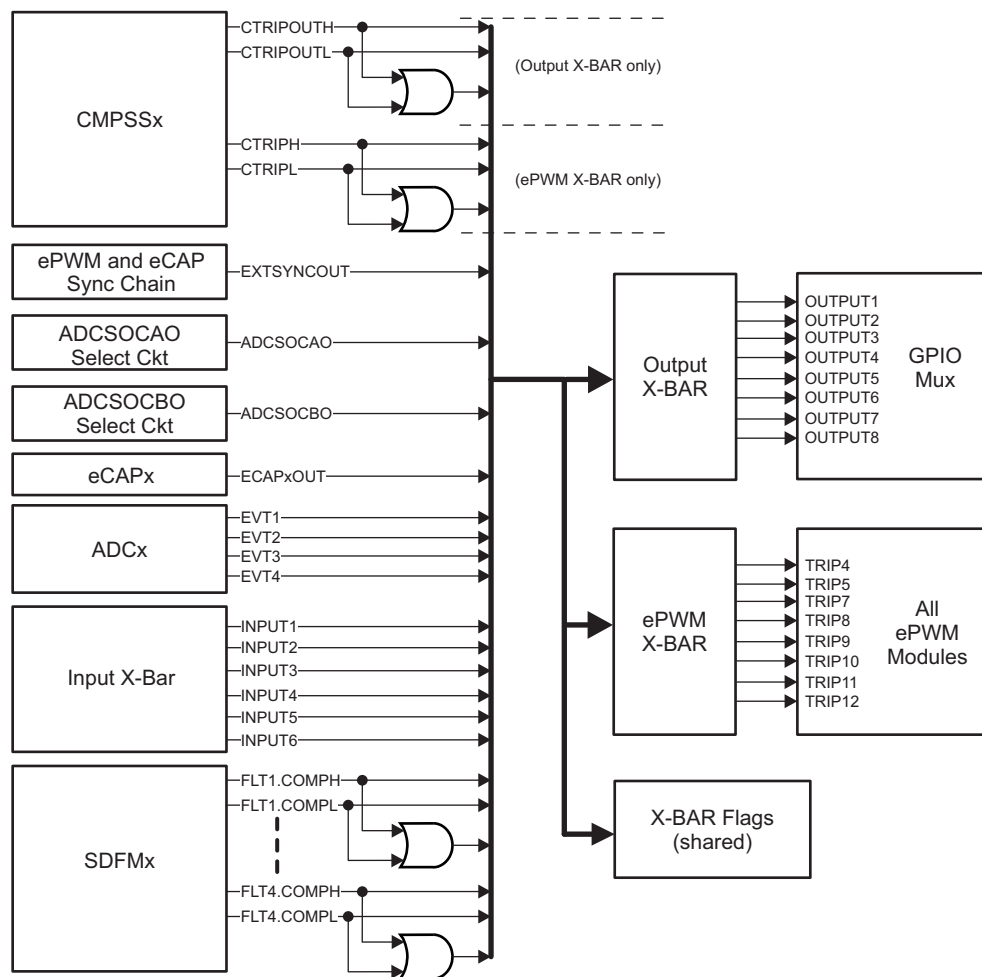
Figure 7-4. ePWM and Output X-BARs Architectures
