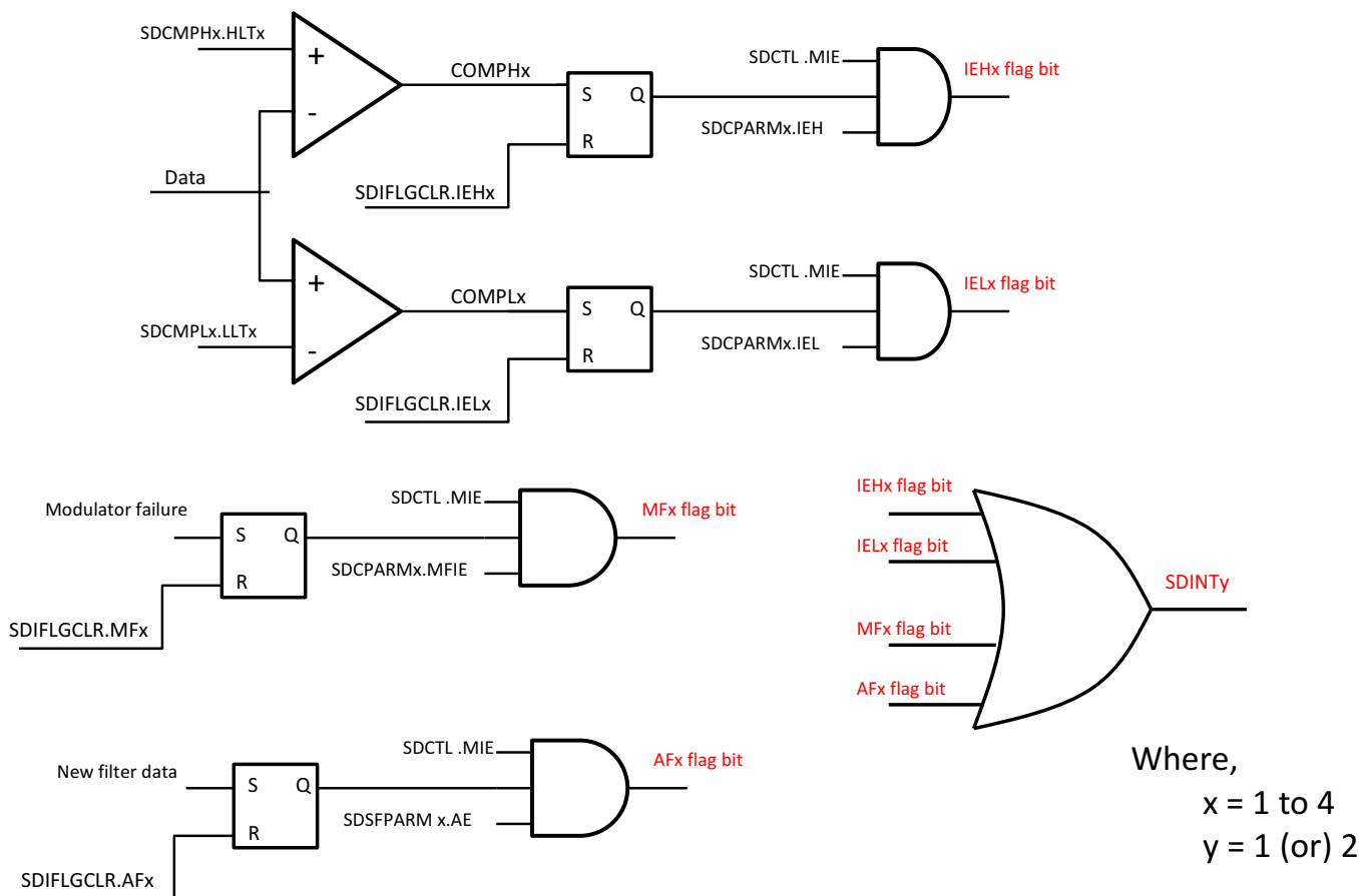
Figure 12-7. SDFM Interrupt Unit
