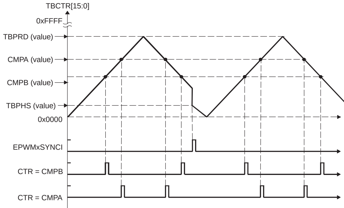
Figure 13-17. Counter-Compare Events In Up-Down-Count Mode, TBCTL[PHSDIR = 0] Count Down On Synchronization Event
