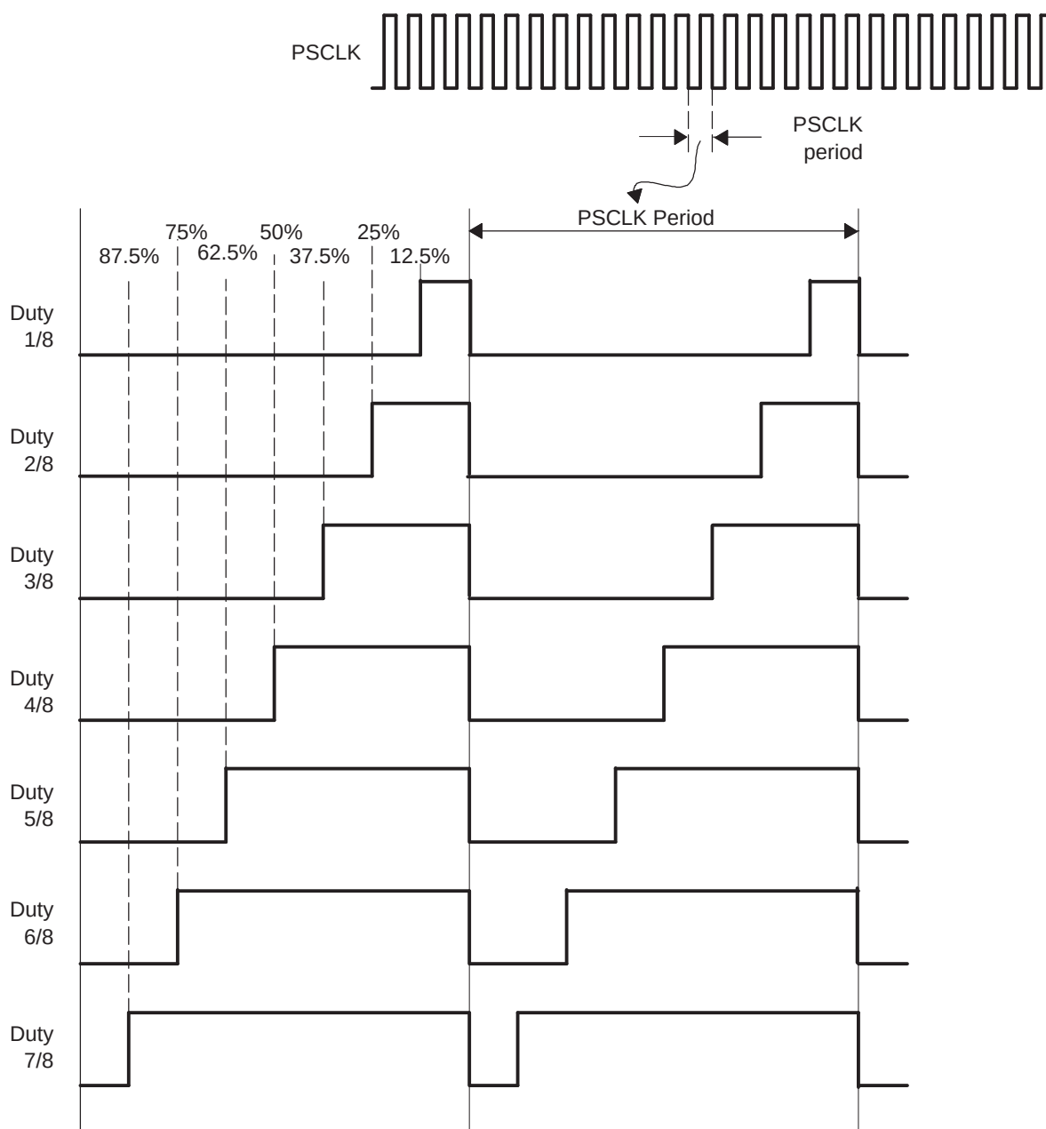
Figure 13-39. PWM Chopper Submodule Waveforms Showing the Pulse Width (Duty Cycle) Control of Sustaining Pulses
