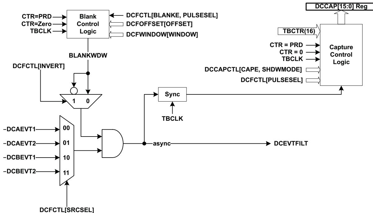
Figure 13-54. Event Filtering
