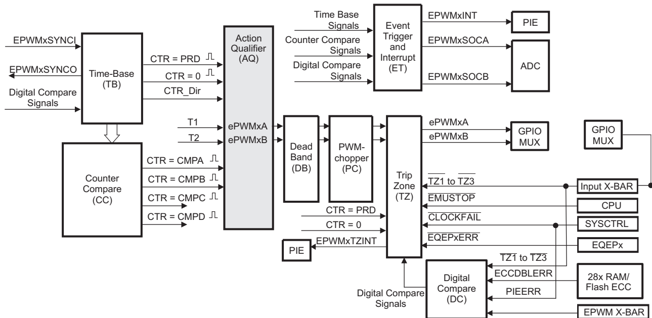
Figure 13-19. Action-Qualifier Submodule
