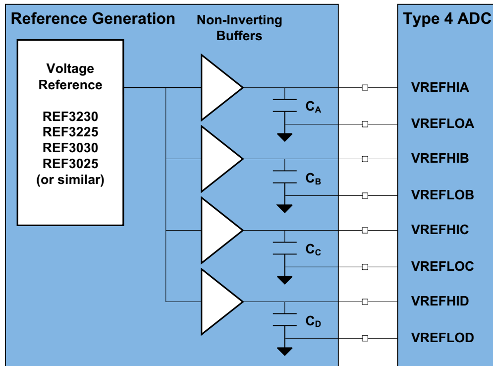
Figure 9-22. Shared Reference System
