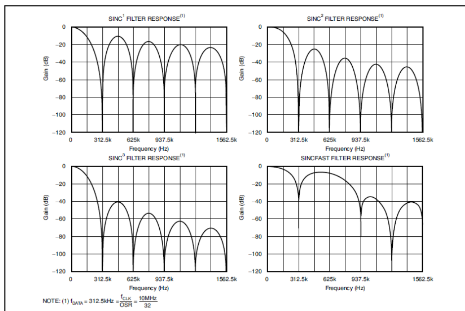
Figure 12-5. Frequency Response of Various Sinc Filters
