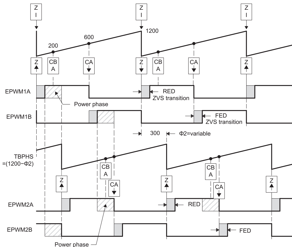
Figure 13-72. ZVS Full-H Bridge Waveforms
