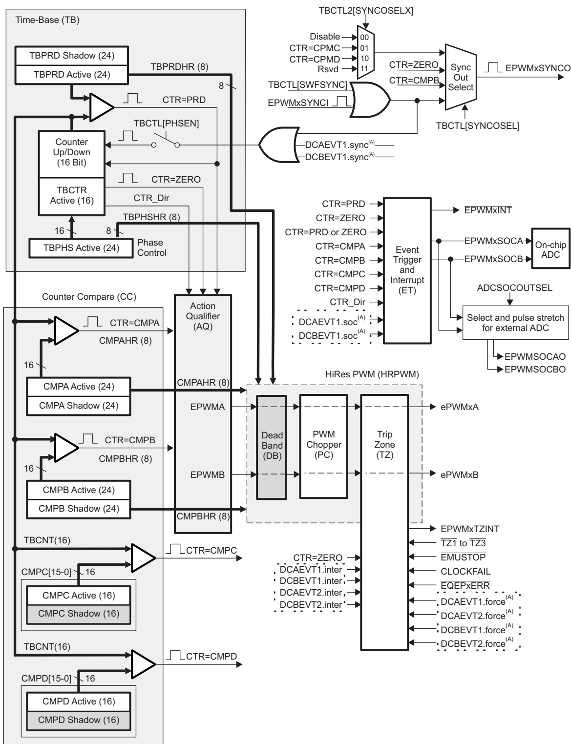
Figure 13-3. ePWM Submodules and Critical Internal Signal Interconnects
