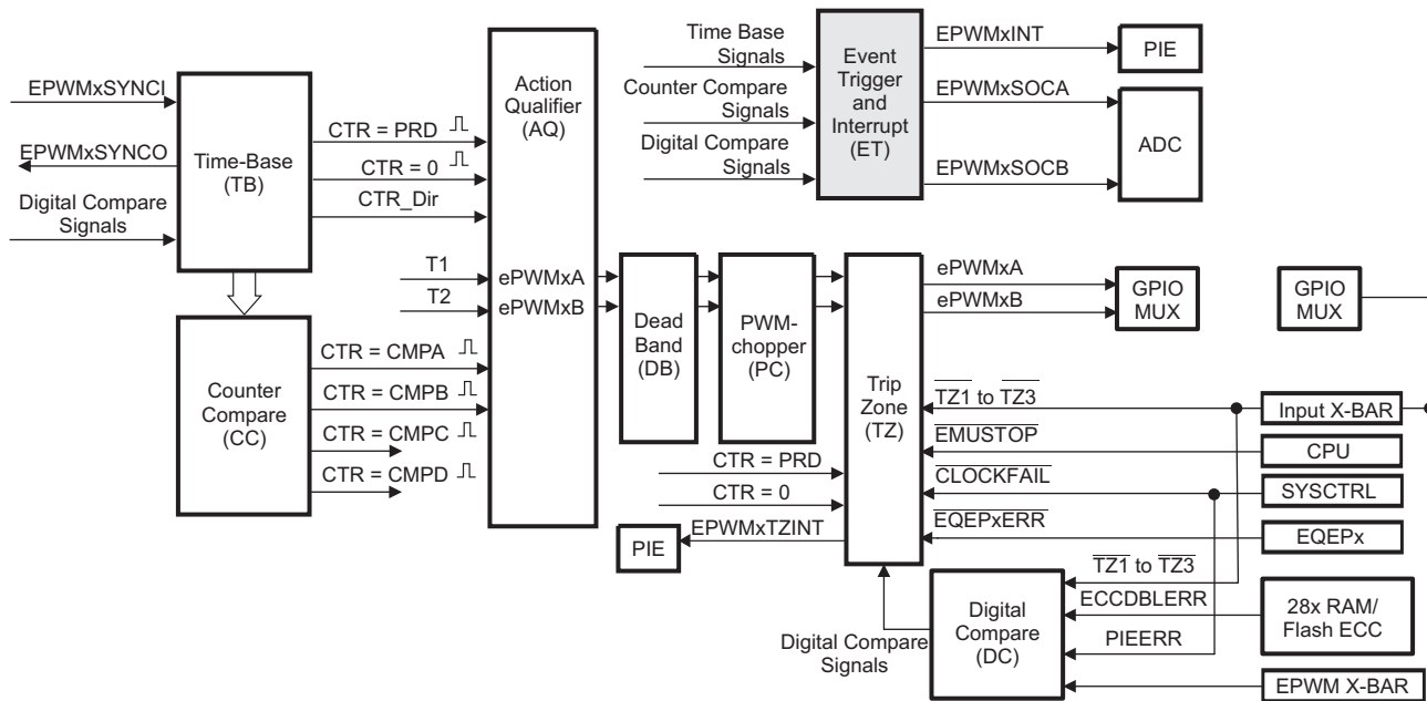
Figure 13-43. Event-Trigger Submodule
