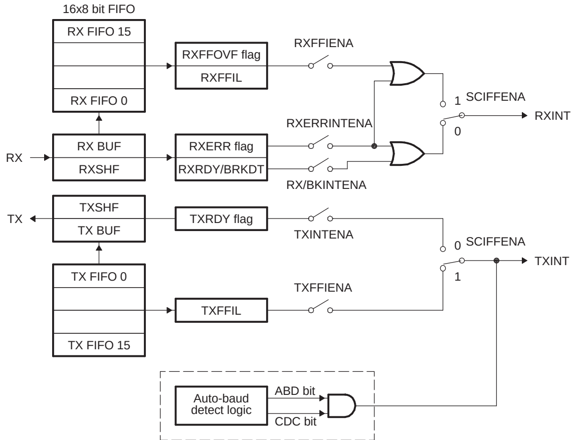
Figure 18-10. SCI FIFO Interrupt Flags and Enable Logic
