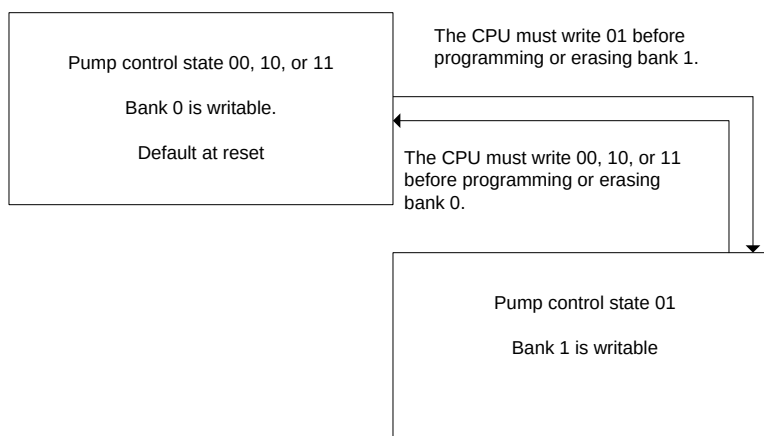
Figure 2-19. PUMP_OWNERSHIP Configuration
