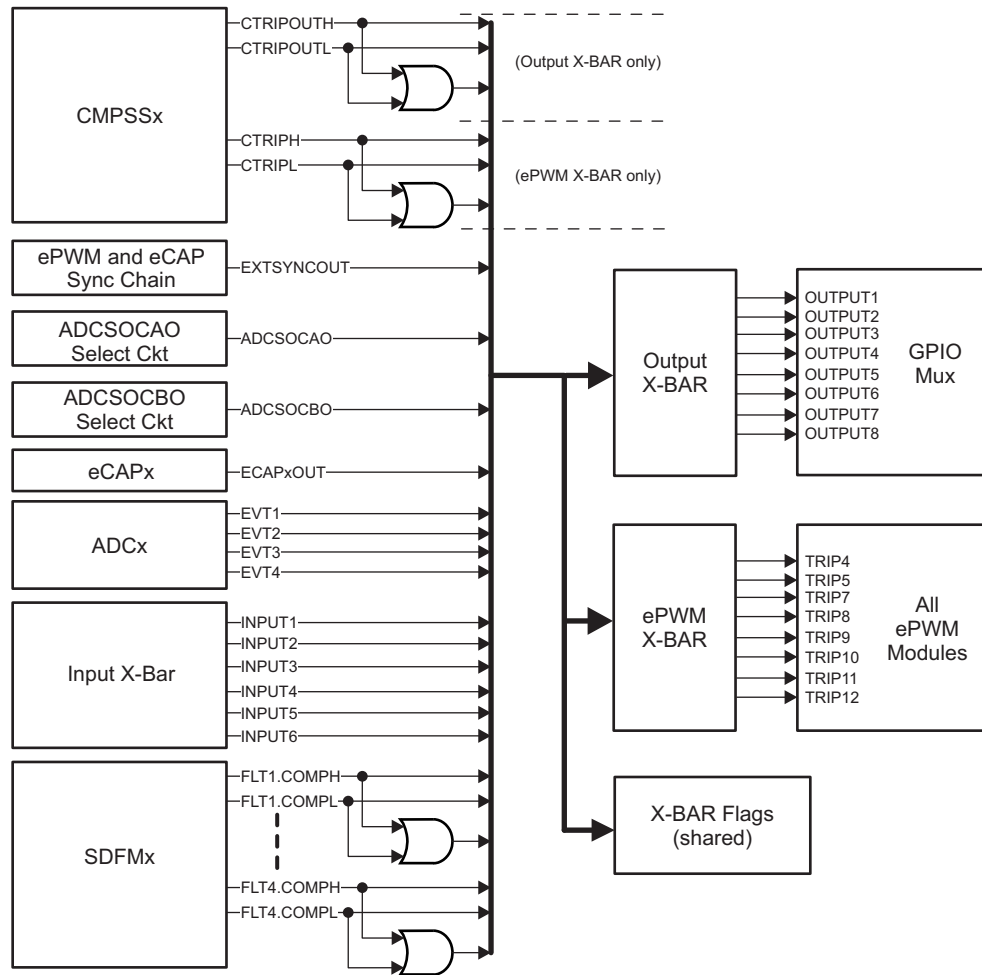
Figure 13-56. EPWM X-BAR
