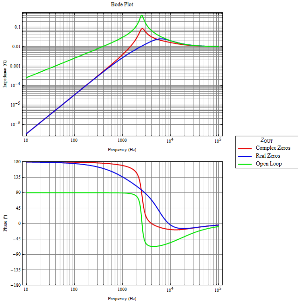
Figure 47: Z_{OUT} Impedance Plots
