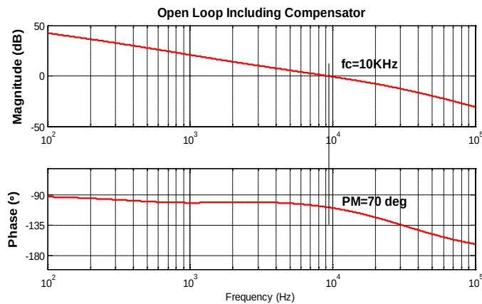
Figure 26: Pole Zero Placement – Bode Plot
