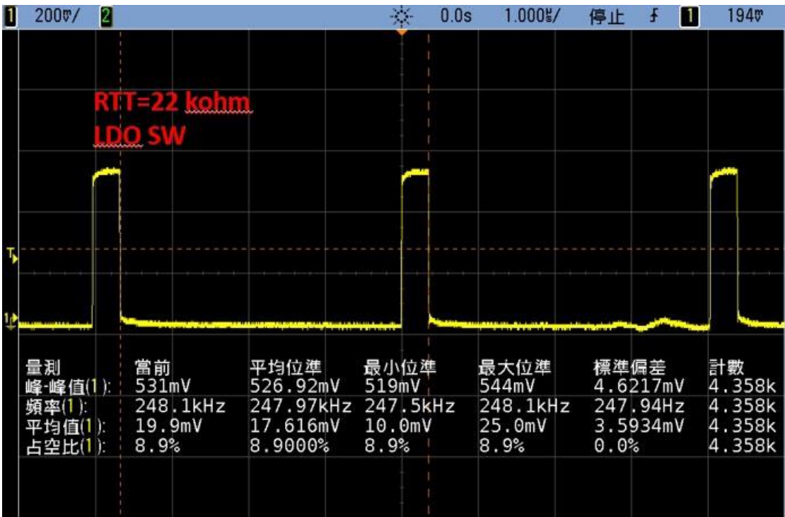
SW waveform
