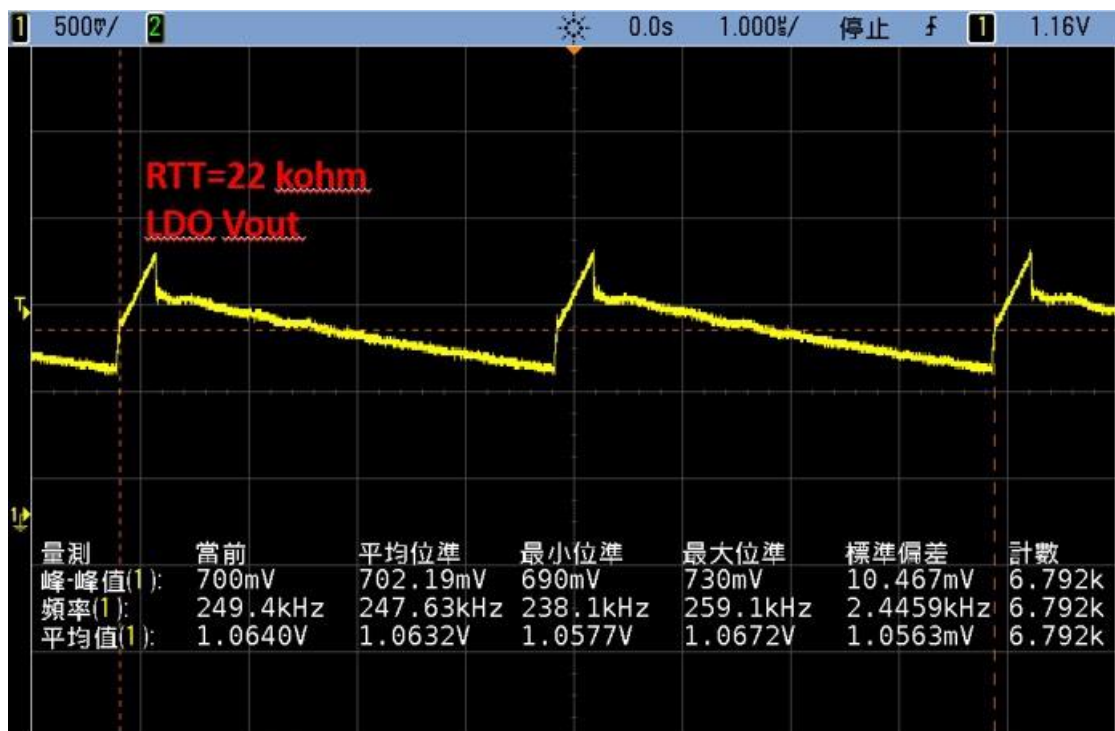
Vout Waveform:
