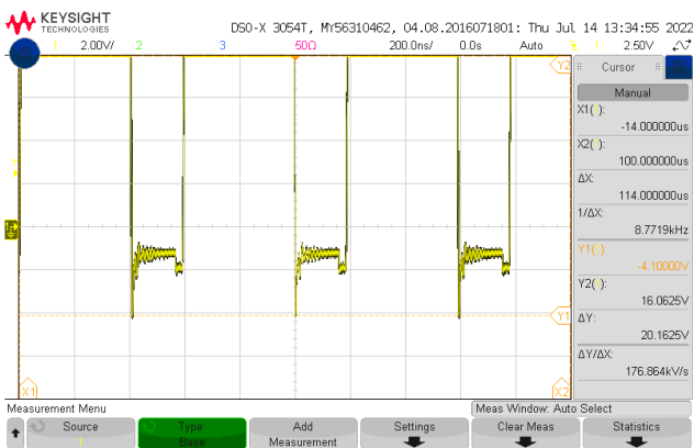
172 DP3 SW pin no Diode at -4.1V
