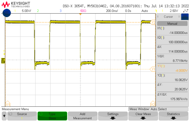
170 w/ Diode and SW at -4.00V
