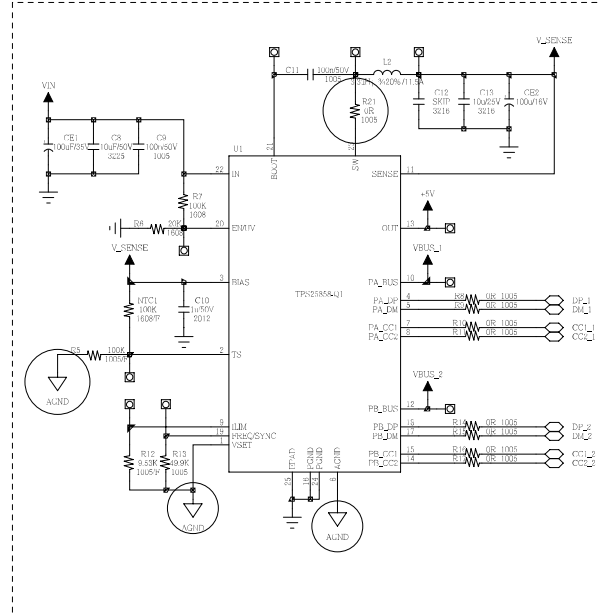
DCDC Circuit
