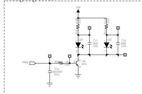
Backlighting Circuit
