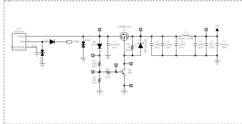
Input Circuit
