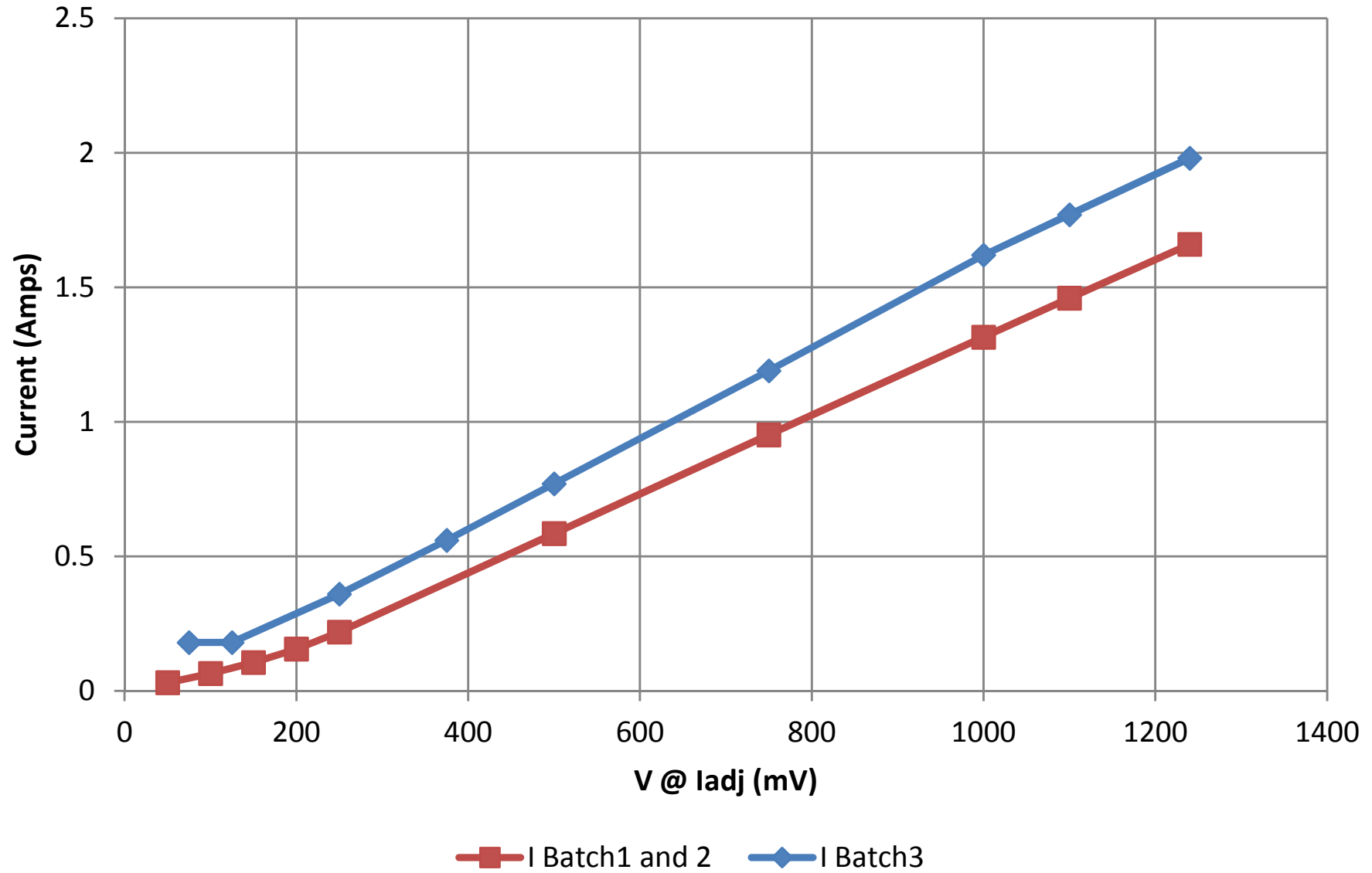
Output current versus Voltage at Iadj LM3409HV
