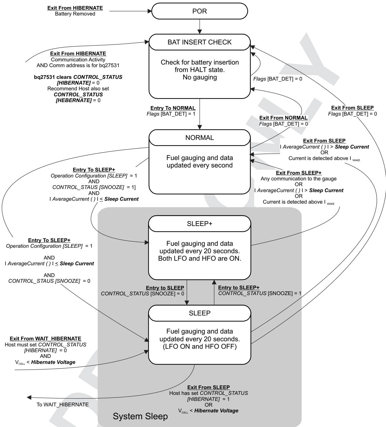
Figure 6-1. Power Mode Diagram—System Sleep
