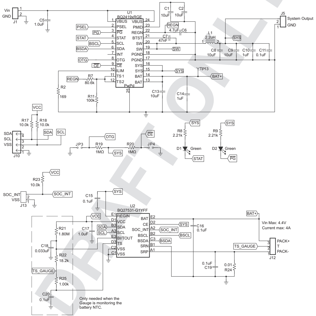
Figure 9-1. Charger Application Schematic
