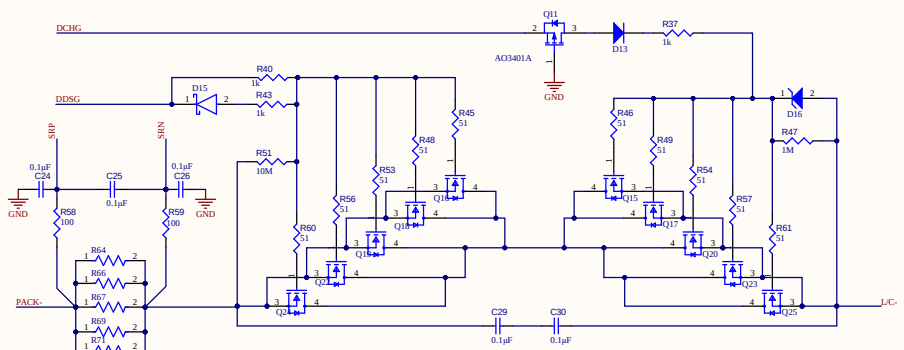
GATE DRIVER
