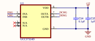
GATE DRIVER
