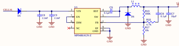
POWER SUPPLY
