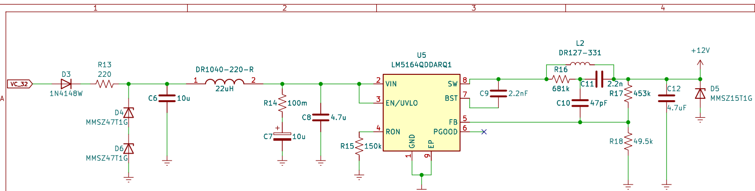
BUCK_1
