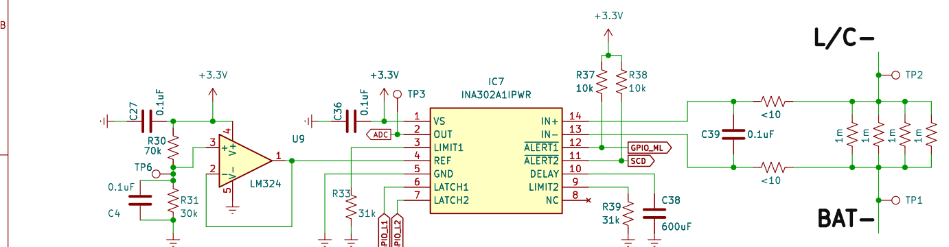
CURRENT_SENSE & SCD_DETECT
