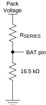
Figure 1. BAT Resistor Divider
