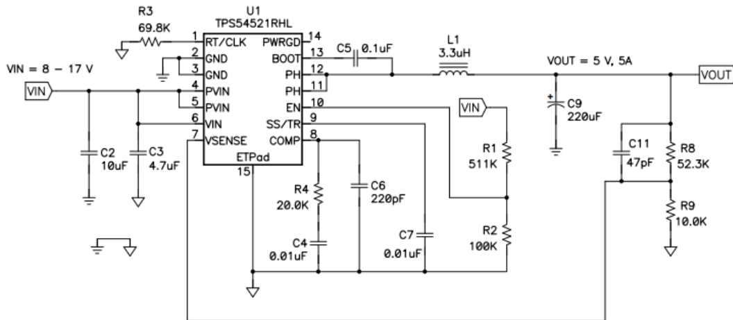
Figure 34. Typical Application Circuit
