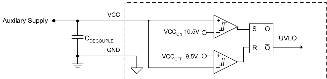
Figure 22. UVLO
