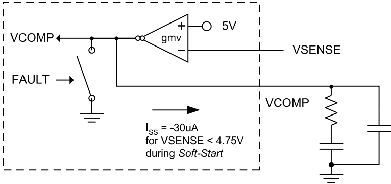
Figure 20. Soft Start
