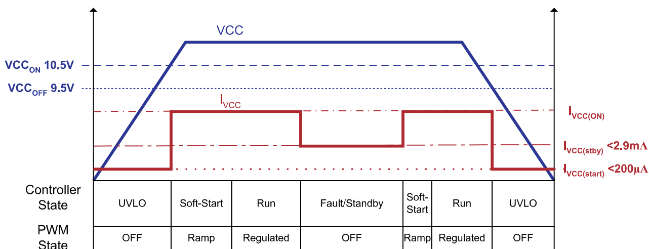
Figure 19. Device Supply States
