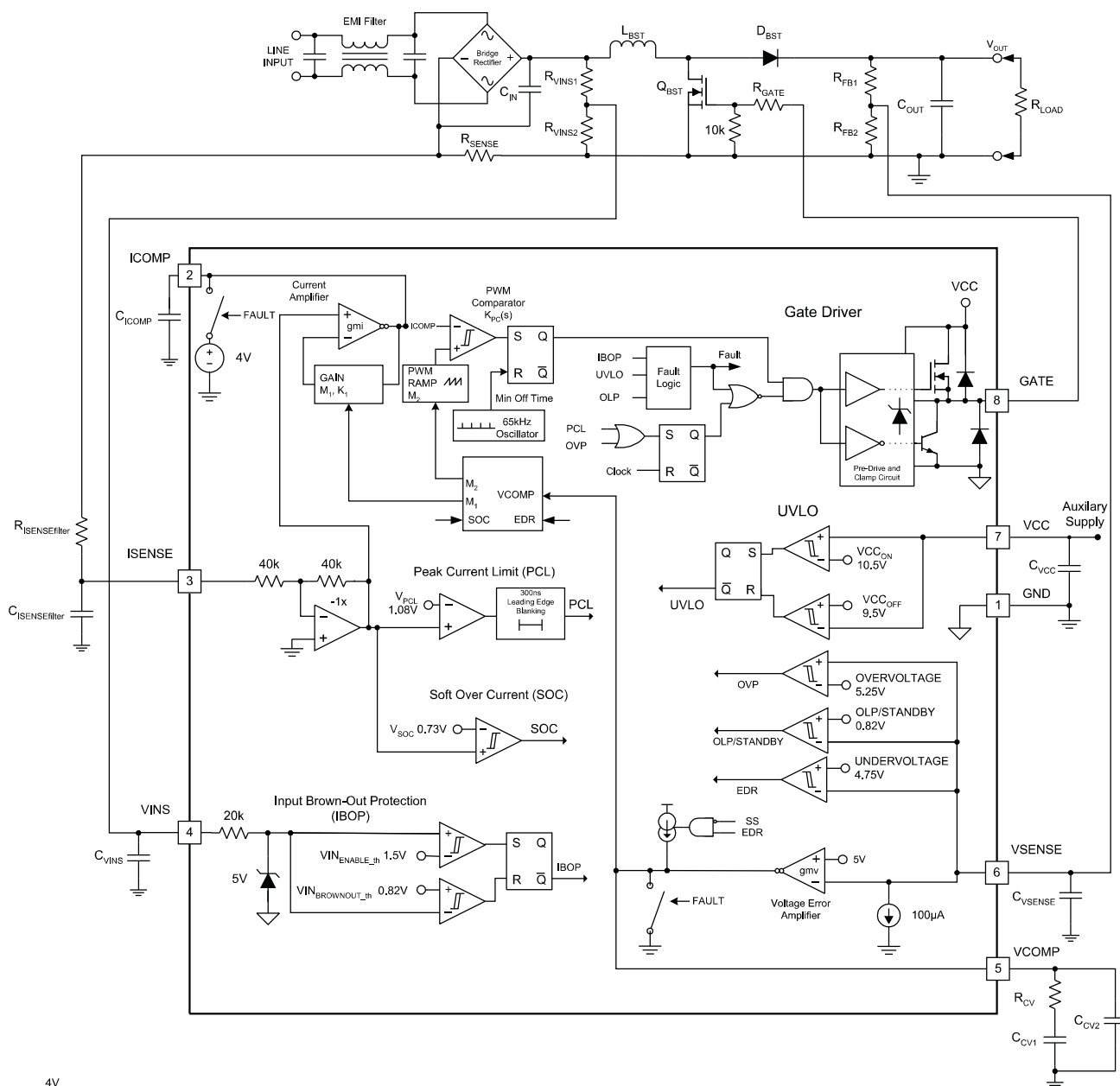
Figure 18. Block Diagram
