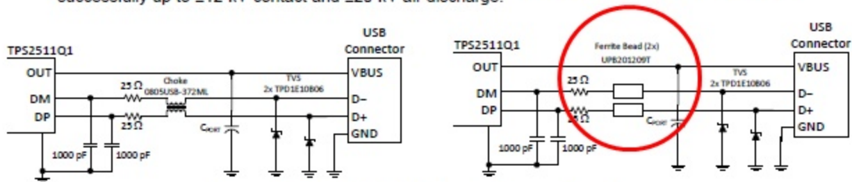
Figure 4. Extended ESD Protection Circuit Examples
