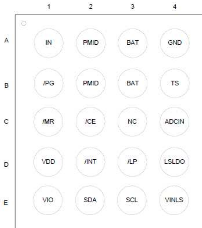
YFP Package 20-Pin DSBGA Top View
