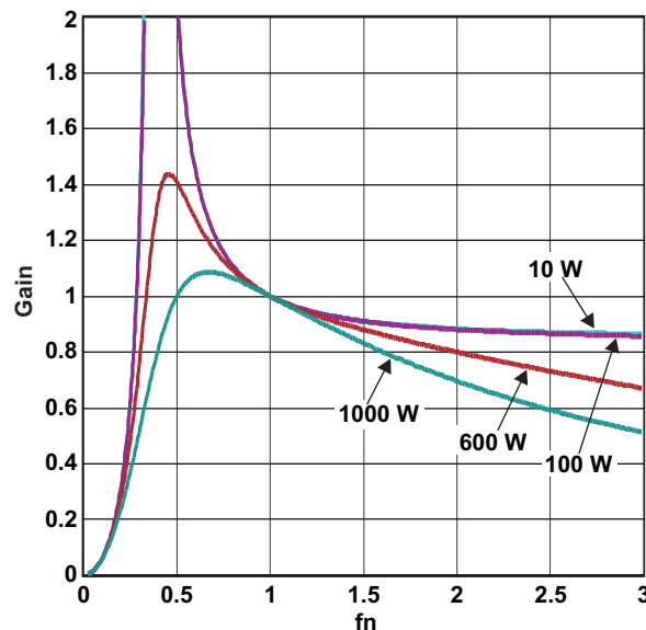
Figure 3. LLC Gain
