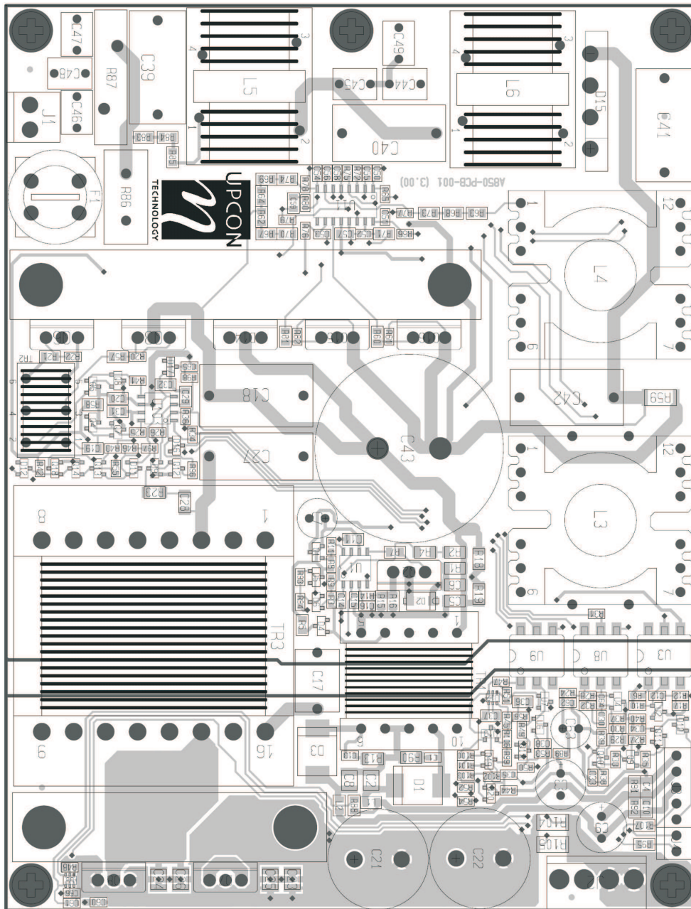
Figure 18. Top Multilayer
