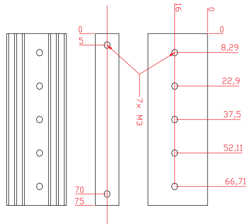
Figure 16. FET Heat-sink
