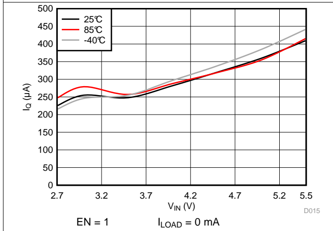
Figure 3. Quiescent Current
