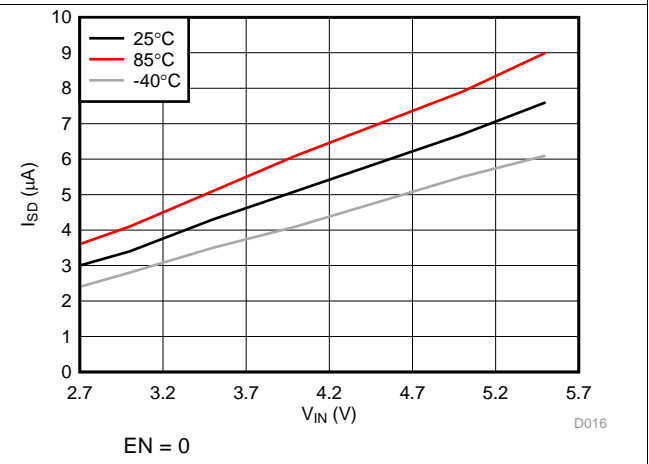
Figure 4. Shutdown Current
