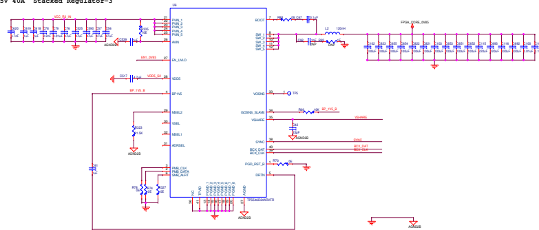
5V to 0.85V 40A Stacked Regulator-3
