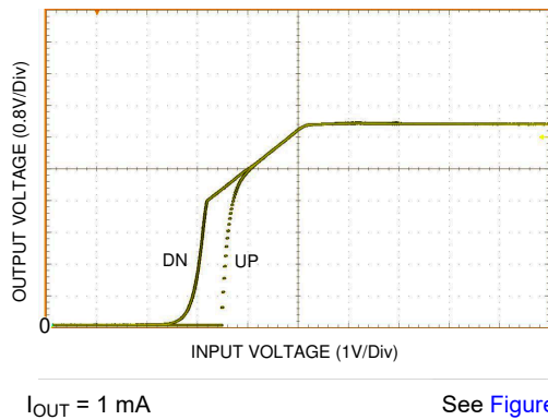
Figure 6-5. UVLO Thresholds
