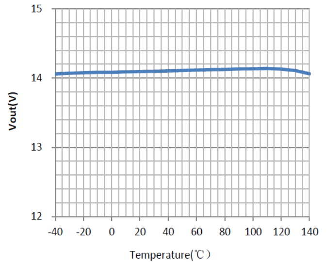
Vout vs. Temperature
