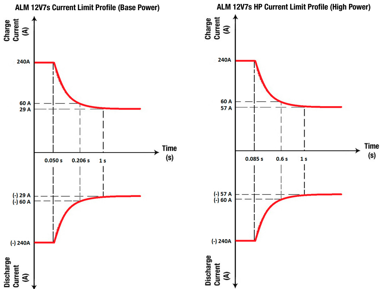
Figure 5 Current Limit Profiles for the ALM 12V7s and ALM 12V7s HP Models
