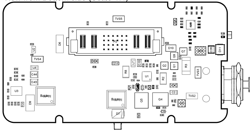
View from Bottom side (Scale 1:1)
