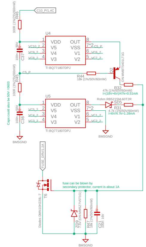
Secondary Protector
