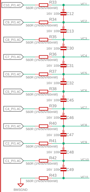
Cell Input Filters for Primary Protector
