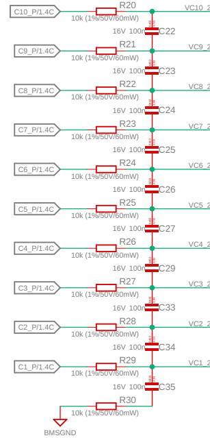
Cell Input Filters for Secondary Protector
