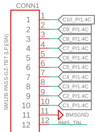
Cell Voltage & Thermistor Connector
