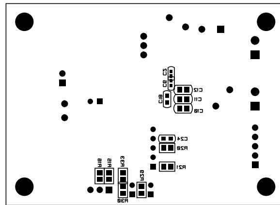
Bottom Silk Screen
