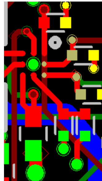
Fuel gauge; Vss bump at center
