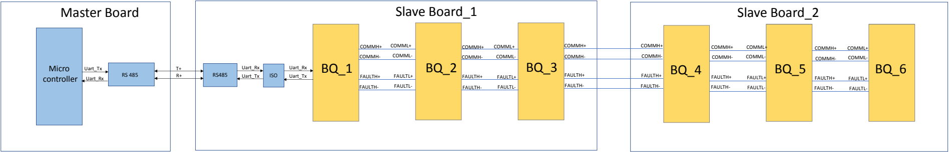
Battery Monitoring Unit (BQ76PL455A-Q1) –Master Slave configuration(RS485)
