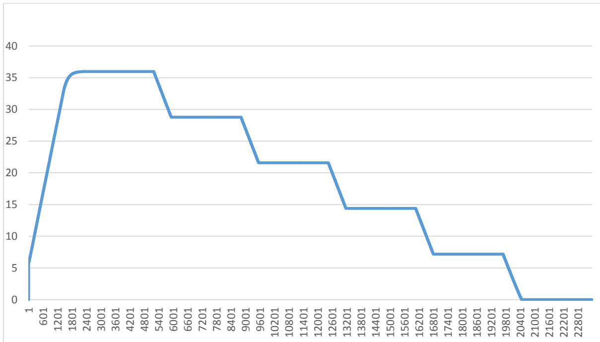
Digatron data (Capacity ah)
