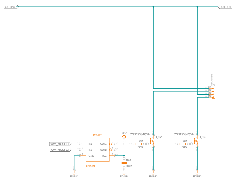
White-Adjust (PWM)
