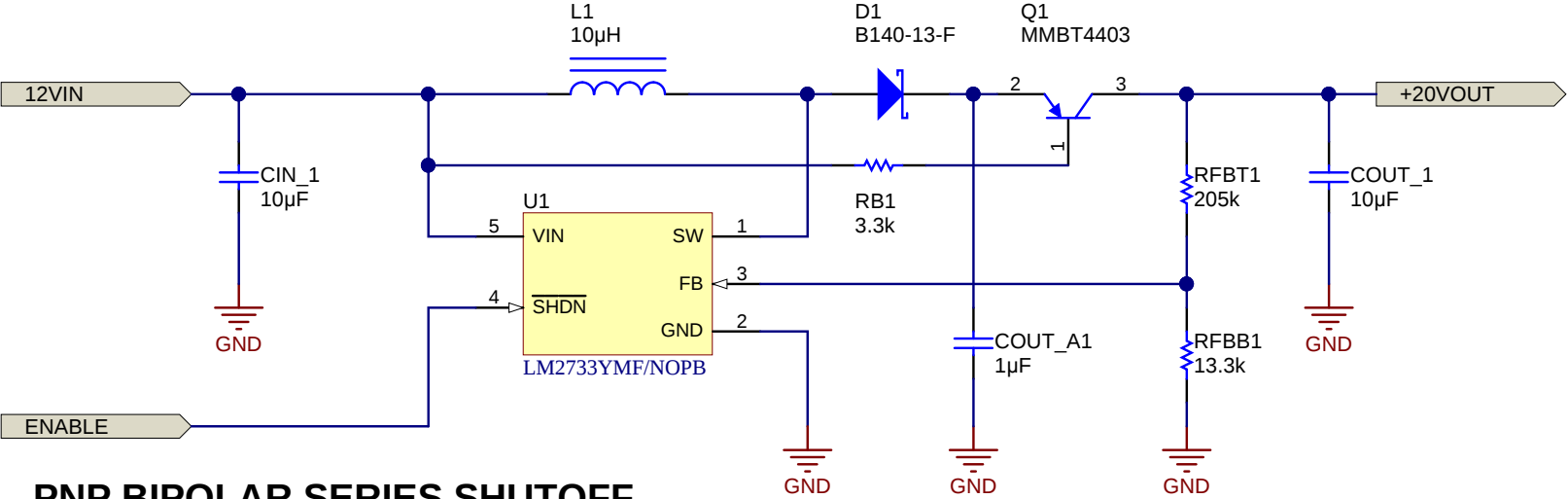
PNP BIPOLAR SERIES SHUTOFF
