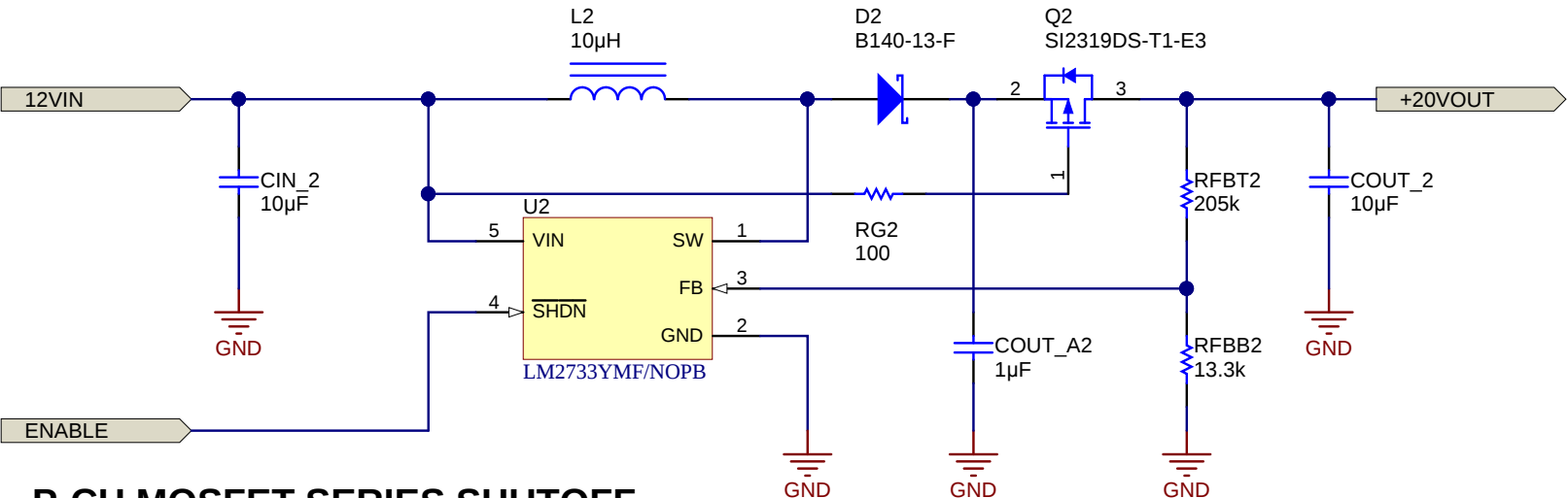
P-CH MOSFET SERIES SHUTOFF
