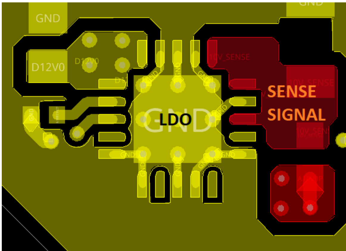
Figure 1 : Sense signal in LDO
