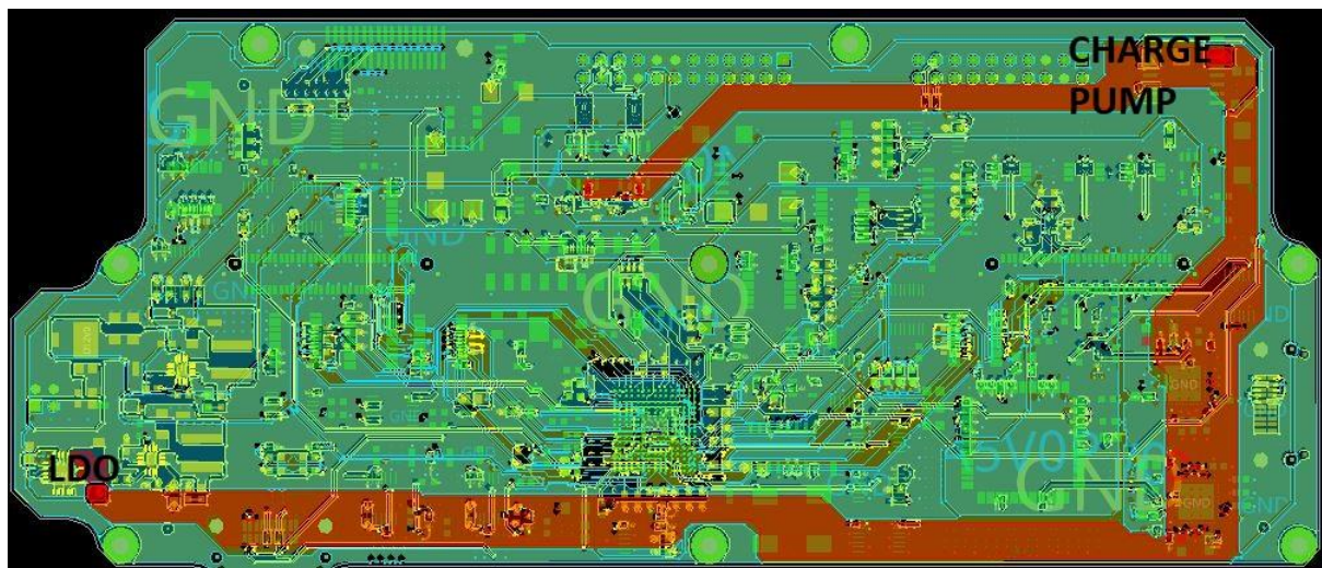
Figure 2 : Placement of LDO and Charge pump ( 16cm between LDO & Charge pump)
