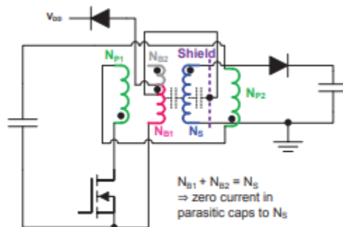
Figure 33. Equivalent schematic of the flyback transformer shown in Figure 32.
