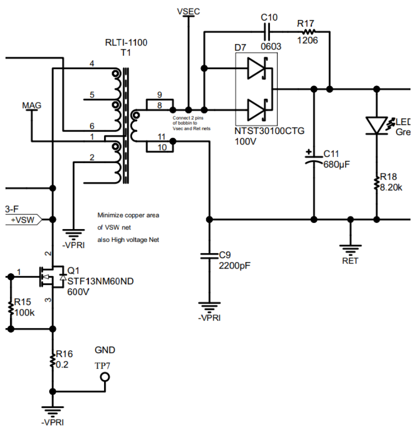
Figure 33. Equivalent schematic of the flyback transformer shown in Figure 32.
