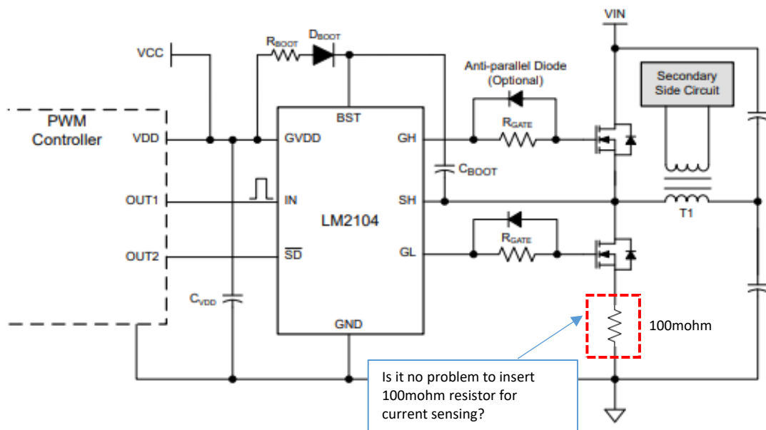
Figure 8-1. LM2104 Driving MOSFETs in a Half-Bridge Converter
