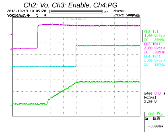
Figure 14: Turn on delay time at 12Vin, 1.2V/60A out (500uS/div)
