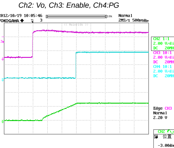
Figure 15: Turn on delay time at 12Vin, 1.5V/60A out (500uS/div)
