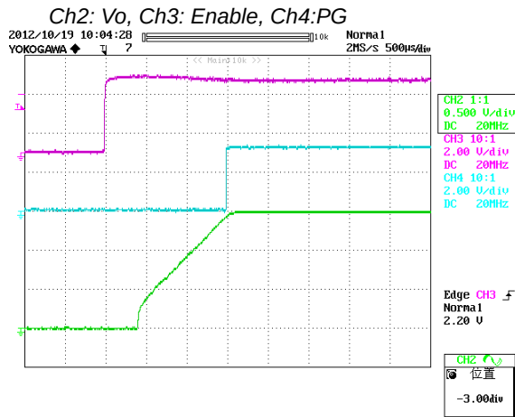
Figure 13: Turn on delay time at 12Vin, 0.9V/60A out (500uS/div)
