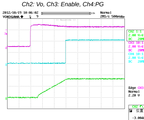
Figure 16: Turn on delay time at 12Vin, 1.8V/60A out (500uS/div)
