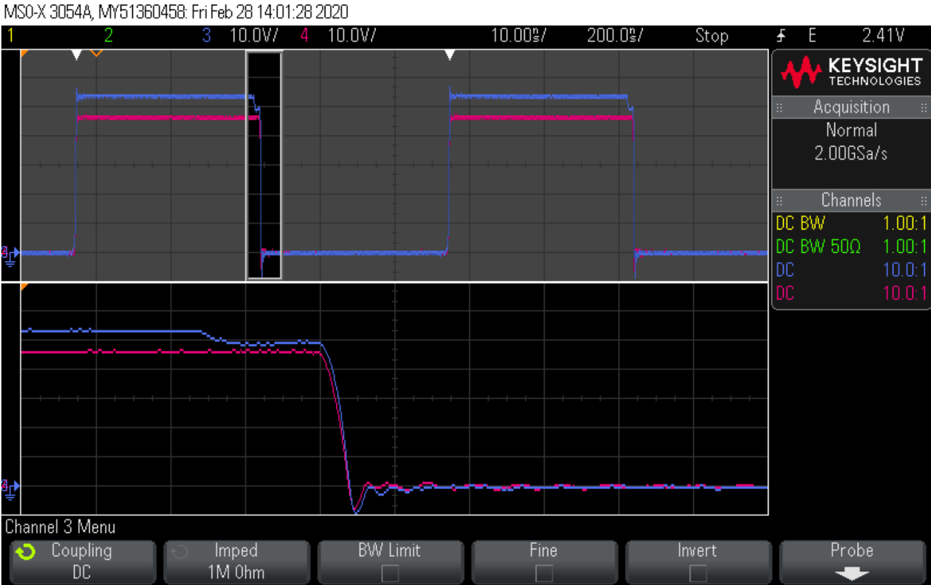
Figure 1 – HO and LO during HS rising, 20nS DT
