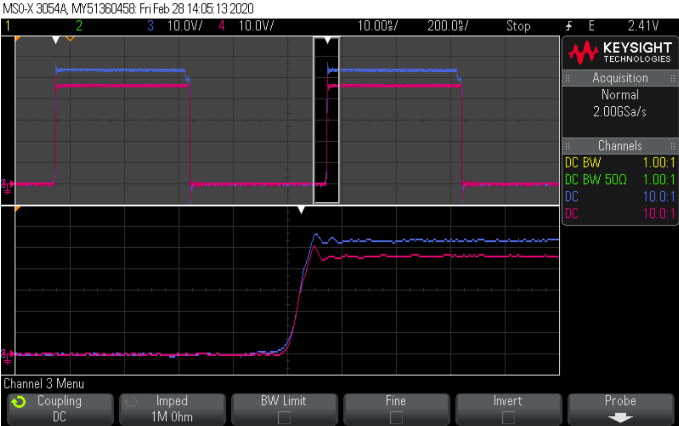
Figure 4 - HO and LO during HS falling, 10nS DT
